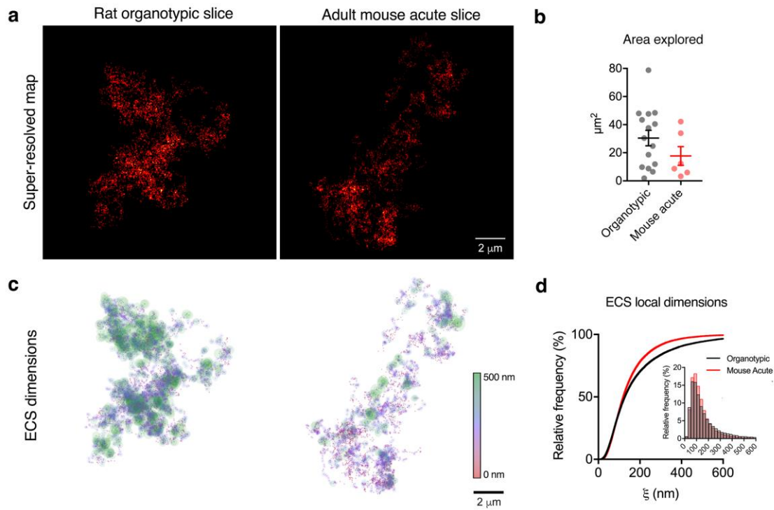
Figure 3: Spatial analysis. a) Examples of super-resolved images obtained from individual SWCNTs freely diffusing in the ECS of a rat organotypic slice and an adult mouse acute slice ( \sim 5000 localizations, respectively). Scale bar = 2 \mu\text{m} . b) Area explored from the totality of SWCNTs tracked in the two models. Data is expressed as mean \pm SEM. c) Maps of local dimensions from the super-resolved SWCNT localizations presented in (a). Maps were drawn by plotting at each localization a circle of size and colour corresponding to the local dimension \xi . Scale bar = 2 \mu\text{m} . d) Cumulative frequency distributions of ECS transverse dimensions \xi from the totality of SWCNTs tracked in this study. Inset: Frequency distribution of the ECS widths, using a bin size of 50 nm.
