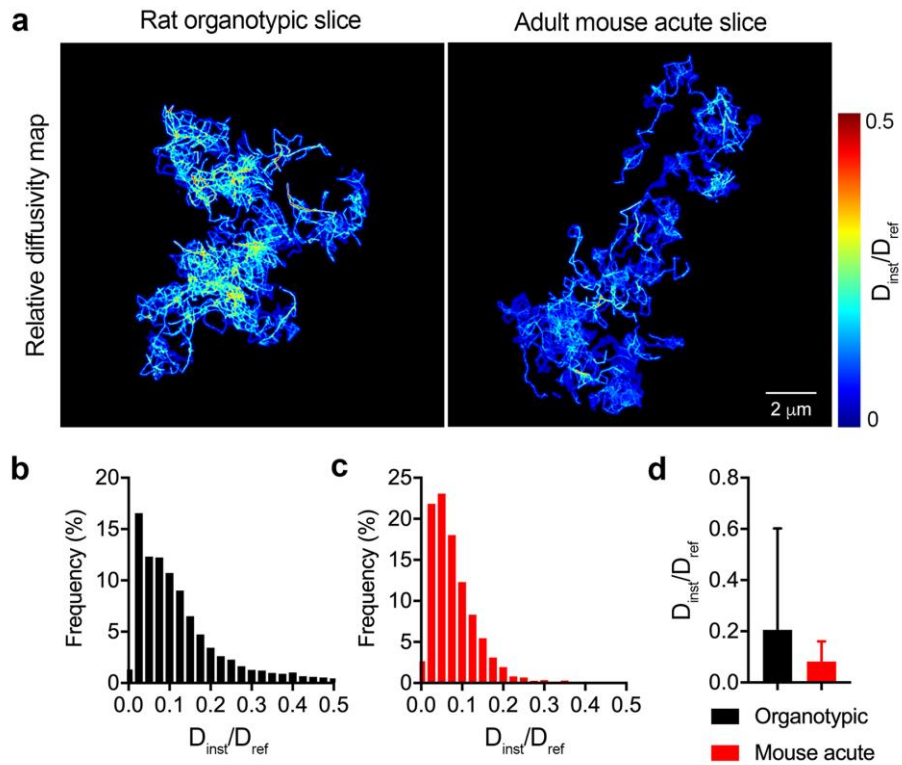
Figure 4: Analysis of ECS dynamics. a) Spatial maps of the instantaneous relative diffusivity coefficients obtained from individual SWCNTs freely diffusing in the ECS of a rat organotypic slice and an adult mouse acute slice. b and c) Frequency distributions of instantaneous relative diffusivity coefficients calculated over the totality of SWCNTs used in this study (black: organotypic slices; red: mouse acute slices). d) Summary of relative diffusivities calculated over the totality of SWCNTs used in this study (mean \pm SD).
