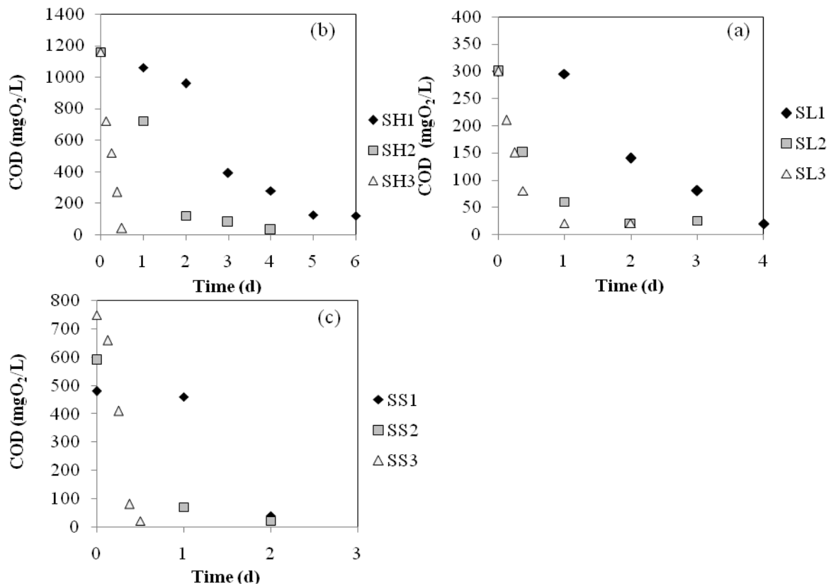
Figure 3: Evolution of Chemical Oxygen Demand COD of SL (a), SH (b) and SS (c) Figure 4 represents the biodegradation kinetics constants of the adaptation of SL, SH and SS at T^\circ=20^\circ\text{C} .
