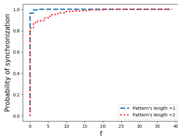
Fig. 8. \frac{\# \text{ successful resynchronizations after a time } t}{\# \text{ total number of runs}} for a pattern's length equal to 1 and to 2 respectively
