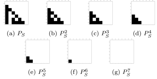
Fig. 4. Powers of P_S^p for p \in [1, 7] , r = 1 . Black squares correspond to non zero entries.
