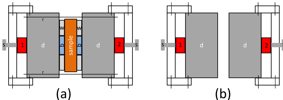
FIG. 1. (Color online) Sketch of the two different configurations of the experimental setup. 1, 2: shear wave transducers. d: delay lines. w: washers playing the role of spacers. b: viscoelastic bond. sample: slab of solid material of interest. s: screw tightening together the transducer and the delay line. r: three threaded rods tightening together the assembly. (a) Mounted setup used to measure the signals reflected and transmitted by the five-layers sandwich. (b) Unmounted setup used to measure the calibration signals.
