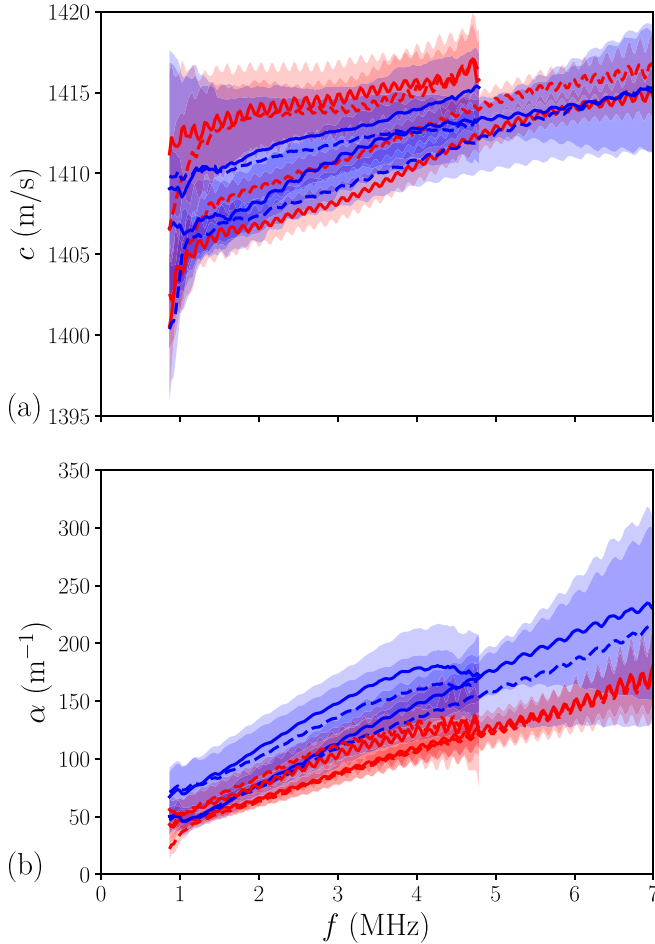
FIG. 9. (Color online) PMMA shear velocity c (a) and attenuation \alpha (b). Each pair of neighbouring (solid and dashed) curves of the same color correspond to two realizations in the same experimental conditions (same sample, same pair of transducers). The uncertainty associated to the determination of c and \alpha by error minimisation is represented as an extra thickness in light colors on both sides of the solid curves (see Appendix B 1).
