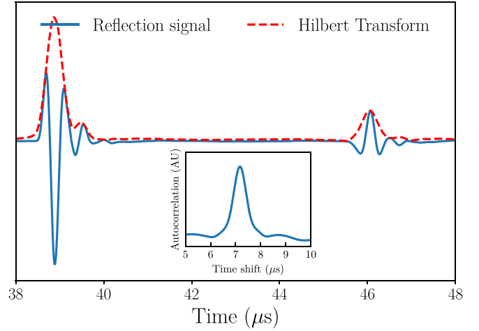
FIG. 11. (Color online) Zoom on the reflection signal (solid blue curve) corresponding to a 5 mm thick sample of PMMA and a pulse excitation at f_c = 2.22 MHz central frequency. Red dashed curve: Hilbert transform. Inset: Autocorrelation of the Hilbert transform of the reflection signal.
