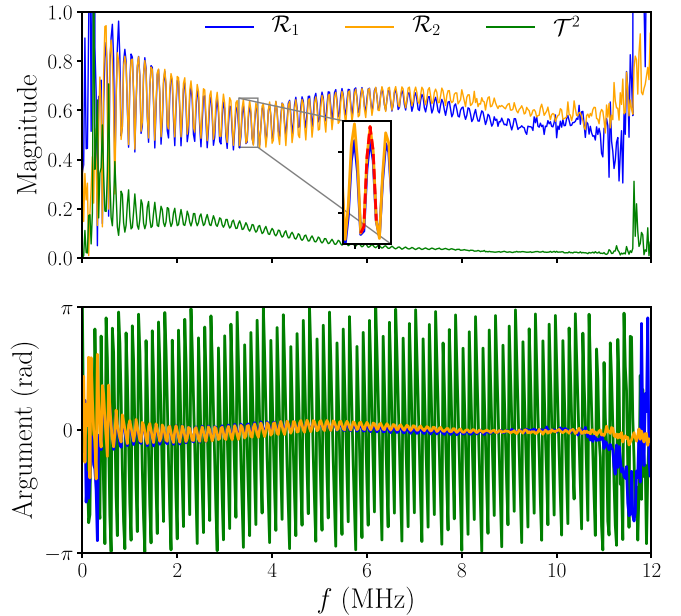
FIG. 3. (Color online) Variation as a function of frequency of the magnitude and argument of \mathcal{R}_1 and \mathcal{R}_2 and of the square of \mathcal{T} determined experimentally using Eq. (1) for the 5 mm thick sample of PMMA and a pulse excitation at f_c = 4.18 MHz central frequency. Inset: zoom on the oscillations of \mathcal{R}_1 and \mathcal{R}_2 . An example of portion of signal along which the averaged error function defined by Eq. (13) is calculated is highlighted as a red dashed curve.
