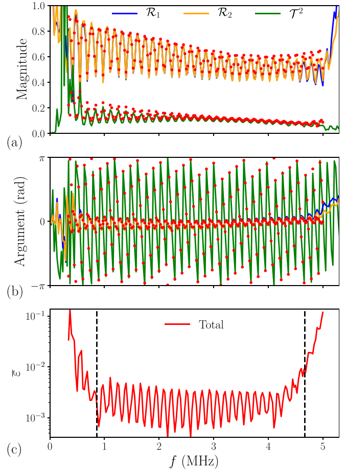
FIG. 7. (Color online) Variations vs frequency of (a) the magnitude and (b) the argument of the measured reflection coefficients \mathcal{R}_1 (blue curve), \mathcal{R}_2 (orange curve), and squared transmission coefficient \mathcal{T}^2 (green curve) defined by Eq. (1) for the 5 mm thick sample and a pulse excitation at f_c = 2.22 MHz central frequency. Red symbols: variations vs frequency of R_{12} and T_{12}^2 defined by Eqs. (5) and (8) and computed using the values of G encountered along the branch of solutions A (see Fig. 6). (c) Variation vs frequency of the residual error \min(\bar{\epsilon}) along this branch.
