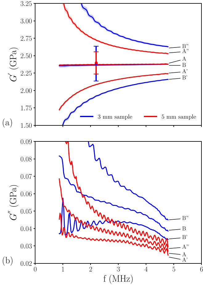
FIG. 6. (Color online) Branches of solutions to the error minimization problem (a) in the (f, G') plane, (b) in the (f, G'') plane. A, A', A'' branches correspond to the 5 mm thick sample and a pulse excitation at f_c = 2.22 MHz. B, B', B'' branches correspond to the 3 mm thick sample and a pulse excitation at f_c = 2.22 MHz. Errorbars in (b) are omitted for clarity purpose. Dot symbols supplied with errorbars: value of G' determined at f_c from time of flight measurement.
