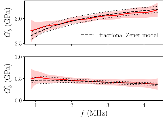
FIG. 10. (Color online) Bond complex shear modulus G_b . Red solid curve with excess thickness in light color: measurements with their uncertainty as defined in Appendix B 1. Black dashed curve: best fit by the fractional Zener model. The black dotted curves are the uncertainty boundaries determined from the uncertainties on the parameters of the rheological model [Eq. (A1)].
