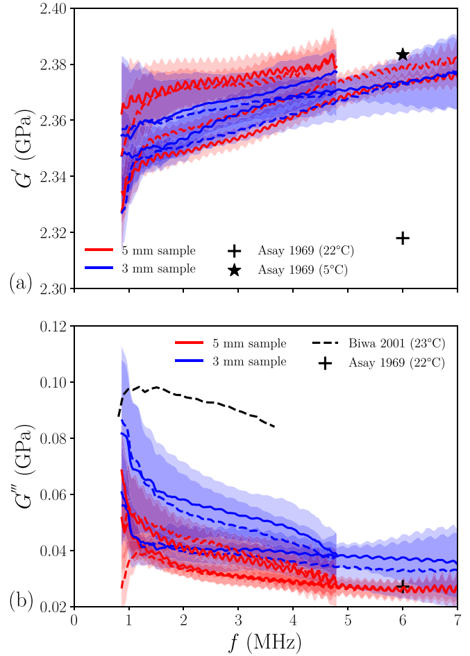
FIG. 8. (Color online) PMMA shear modulus: comparison with literature. Each pair of neighbouring (solid and dashed) curves of the same color correspond to two realizations in the same experimental conditions (same sample, same pair of transducers). The uncertainty associated to the determination of G' and G'' by error minimisation is represented as an extra thickness in light colors on both sides of the solid curves (see Appendix B 1). Biwa et al. (2001) measured G' = 2.25 GPa in the frequency range 2–5 MHz at 23 °C.
