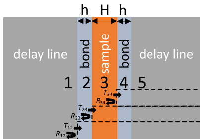
FIG. 4. (Color online) Sketch and notations for the interference model.
