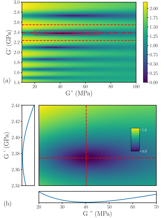
FIG. 5. (Color online) (a) Variations in color scale of the decadic logarithm of the relative averaged error function \log[\bar{\varepsilon}/\min(\bar{\varepsilon})] in the vicinity of its absolute minimum \min(\bar{\varepsilon}) at f = \omega/2\pi = 2.22 MHz as function of the real and imaginary parts G' and G'' of the sample complex shear modulus G for the 5 mm thick sample and a pulse excitation at f_c = 2.22 MHz central frequency. The red dot-dashed line indicates the value of G' deduced from time of flight measurement (see text) and the dashed lines its uncertainty. The red solid frame indicates the enlarged area shown below. (b) Enlarged area. The red dashed lines indicate the values of G' and G'' for which \bar{\varepsilon} is minimum. Graphs below and on the left: variations of \bar{\varepsilon} versus G' and G'' in linear scales along the red dashed lines.
