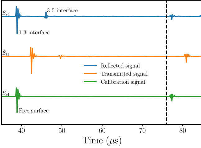
FIG. 2. (Color online) Reflection, transmission, and calibration signals corresponding to the 5 mm thick sample of PMMA and a pulse excitation at f_c = 2.22 MHz central frequency. The vertical dashed line indicates the end of signal analysis. Beyond this time, other echoes having experienced a reflection on one transducer-delay line interface are visible. Interface designation refers to labels defined in Fig. 4.
