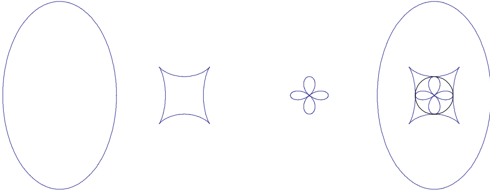
Figure 7. (a) The ellipse (b) \mathcal{H}_{h-4} (c) \mathcal{P}_0(\mathcal{H}_{h-4}) ; (d) These curves and C(0_{\mathbb{R}^2}; 1)
