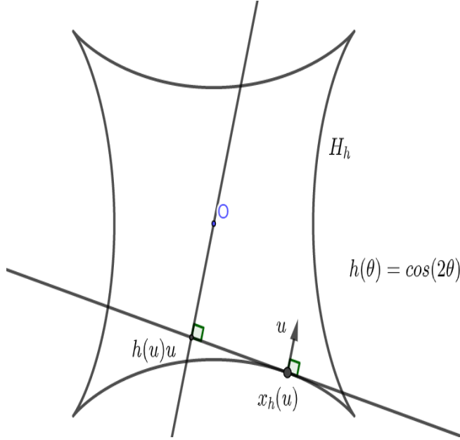
Figure 2. Plane hedgehog with C^2 -support function
