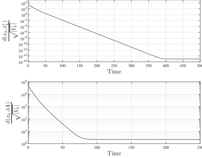
Fig. 3. Evolution of the normalized open distance between network state and average reference input |V_k|^{-1/2} d(x_k, \bar{u}) and between network state and point of interest |V_k|^{-1/2} d(x_k, x_k^e) , in the case of time-invariant number of agents n = 200 .
