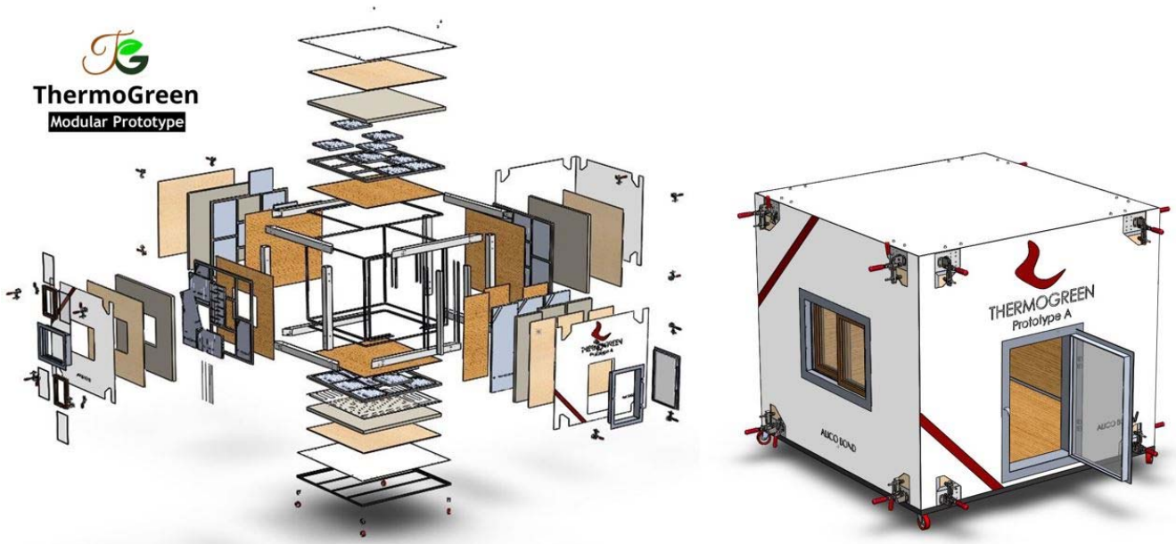
248 Figure 4 Exploded view and logo of the complete assembly of the modular prototype.
