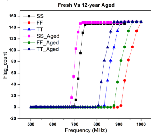
Figure 8 Corner Impact on Flag Count for FIR Filter synthesized at 500MHz for different Corners
