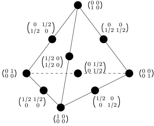
Fig. 3: The 2-discretized probability simplex \mathcal{P}_2(\mathcal{X} \times \mathcal{Y}) for \mathcal{X} = \mathcal{Y} = \{0, 1\} .
