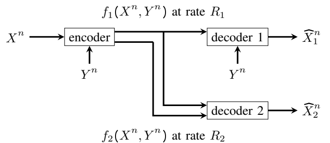
Fig. 1: Source coding when side-information may be present.
