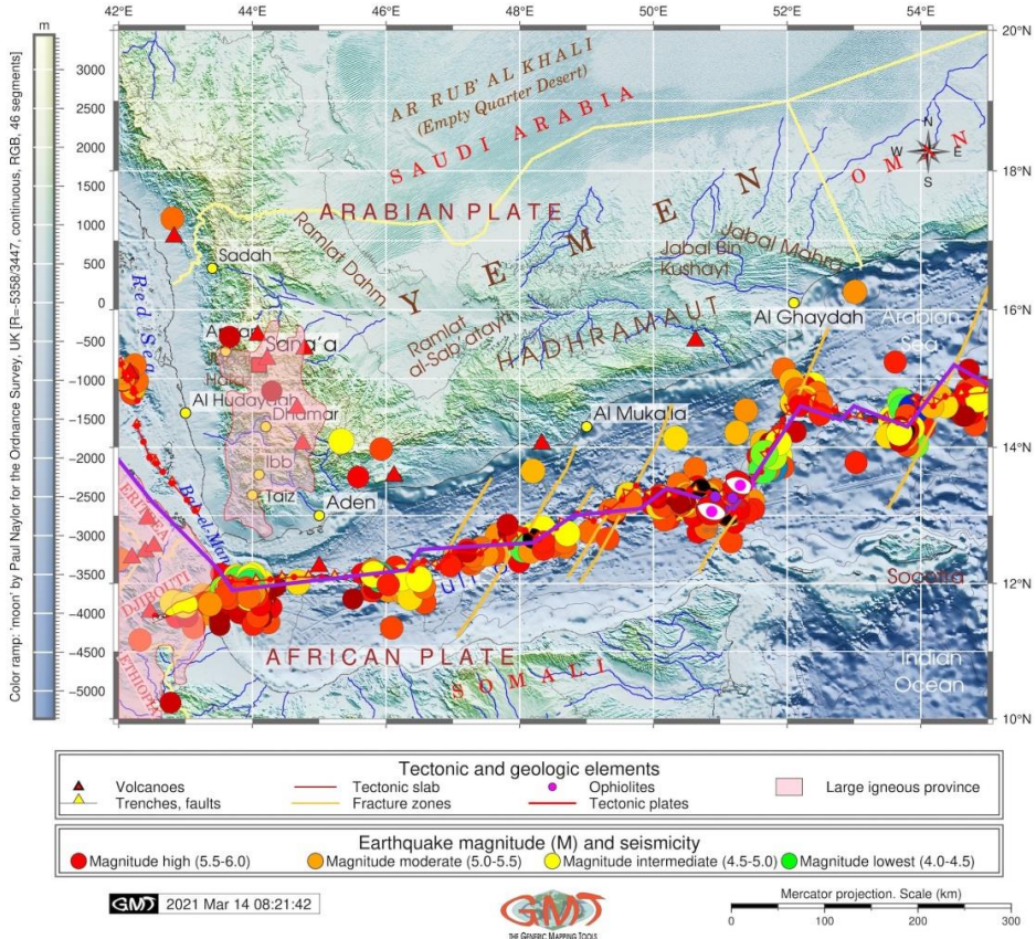
Fig. 4. Earthquakes seismicity in the Gulf of Aden and Yemen. Data: IRIS. Mapping: GMT. Source: author.
