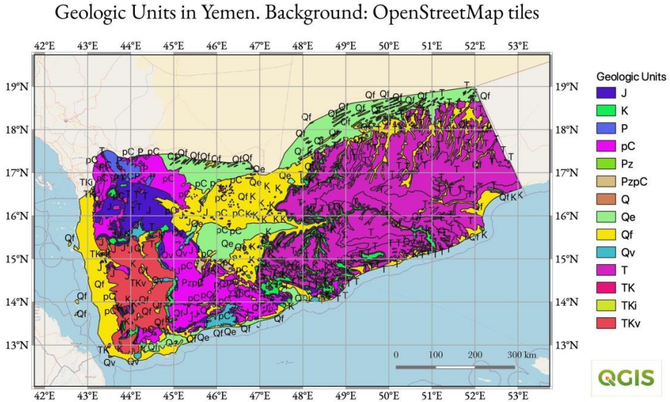
Fig. 3. Geologic Units, Volcanics and Intrusives in Yemen. Data: USGS. Mapping: QGIS. Source: author.
