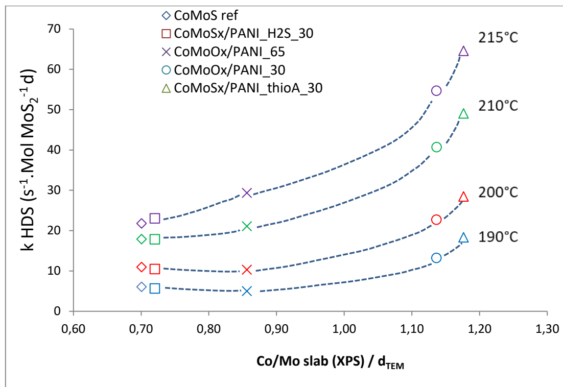
Figure 9: Normalized HDS rate constants k_{\text{HDS}} versus the (\text{Co}/\text{Mo})_{\text{edges+corner}} atomic ratio at different temperatures.
