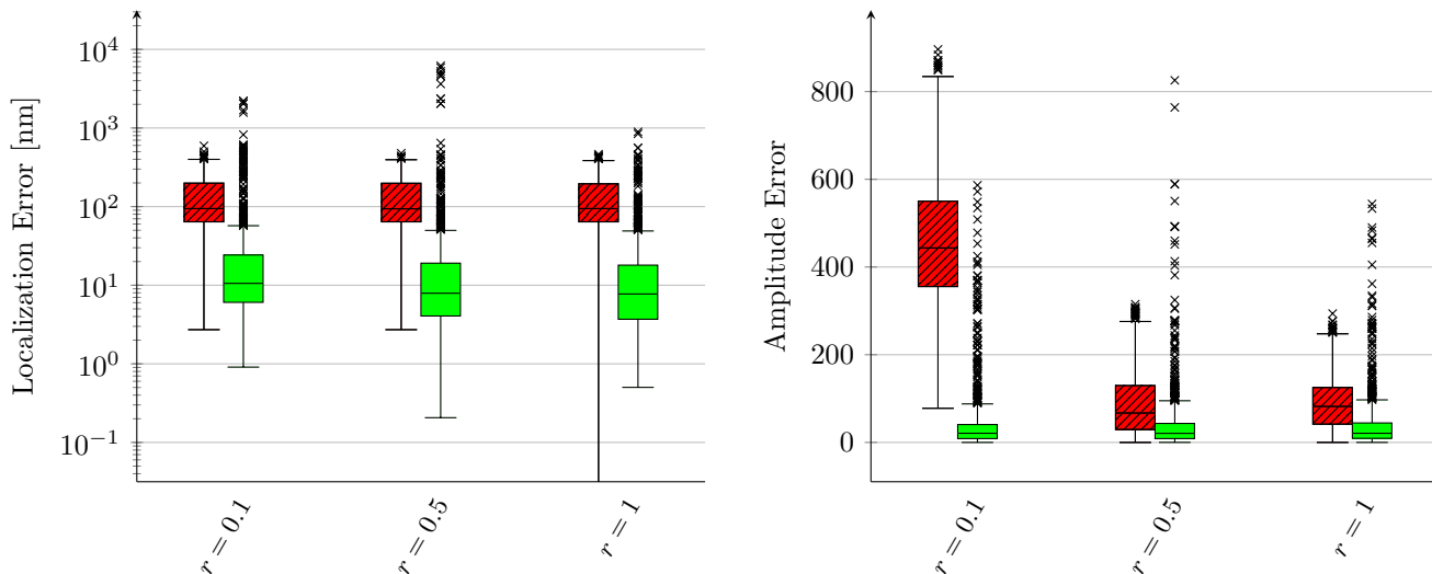
Figure 8: Box plots of the localization (left) and amplitude (right) error for different noise levels. Three noise levels are displayed with r = 0.1, 0.5 , and 1 . For each case, the left box plot (hatched) corresponds to the initial positions/amplitudes and the right box plot (solid) corresponds to the refined positions/amplitudes. Note that the estimated amplitudes were scaled by r^{-1} to compare with the same ground-truth. For the box plots of the localization error after refinement (solid), we set the upper whiskers to 50\text{nm} so as to consider any larger error as outliers. This is in line with the expected 3D localization error in SMLM [6]. This bound is not relevant for the initial errors (hatched) as they are too large. For the hatched box plots, we thus set the default upper whiskers to Q3 + 1.5\text{IQR} , where \text{IQR} = (Q3 - Q1) is the interquartile range and Q1, Q3 are the 25th and 75th percentile, respectively. Finally, the lower whiskers are always set to the smallest error among all molecules. Outliers are indicated by \times .
