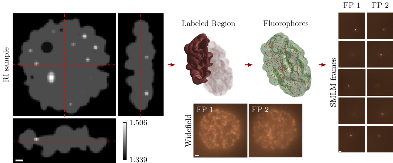
Figure 2: Simulation setup. The RI map, immersed in water ( n_b = 1.339 ), is depicted on the left orthoviews. The sample is populated with fluorescent molecules that belong to the labeled region. They sequentially emit a spherical wave which is then propagated through the sample using the Lippmann-Schwinger model. Two focal planes (with pupil functions) are acquired. The widefield images are generated by summing all SMLM frames. The fluorescence images were saturated for visualization purpose. We display the labeled region with partial transparency so as to make the inner compartments visible. Scale bars: 500nm.
