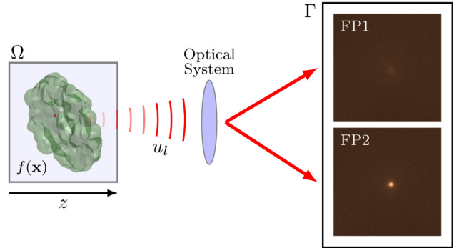
Figure 1: Biplane single-molecule localization microscopy. A fluorophore emits fluorescent light which scatters through the sample. Then, an optical system records the intensity of the total field at two different focal planes.
