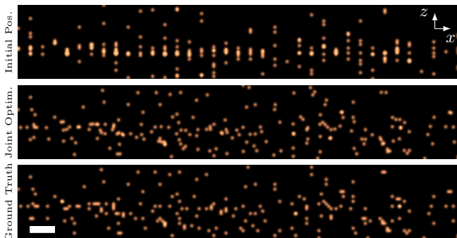
Figure 5: Rendering of localized molecules (Y-projection). Region-of-interest of the projection along Y of the rendered fluorescent volume. From top to bottom: Initial positions, positions refined with the joint-optimization framework, ground-truth. Field-of-view (XZ): (3600 \times 600)\text{nm}^2 . The images were saturated for visualization purpose. Scale bar: 200nm.
