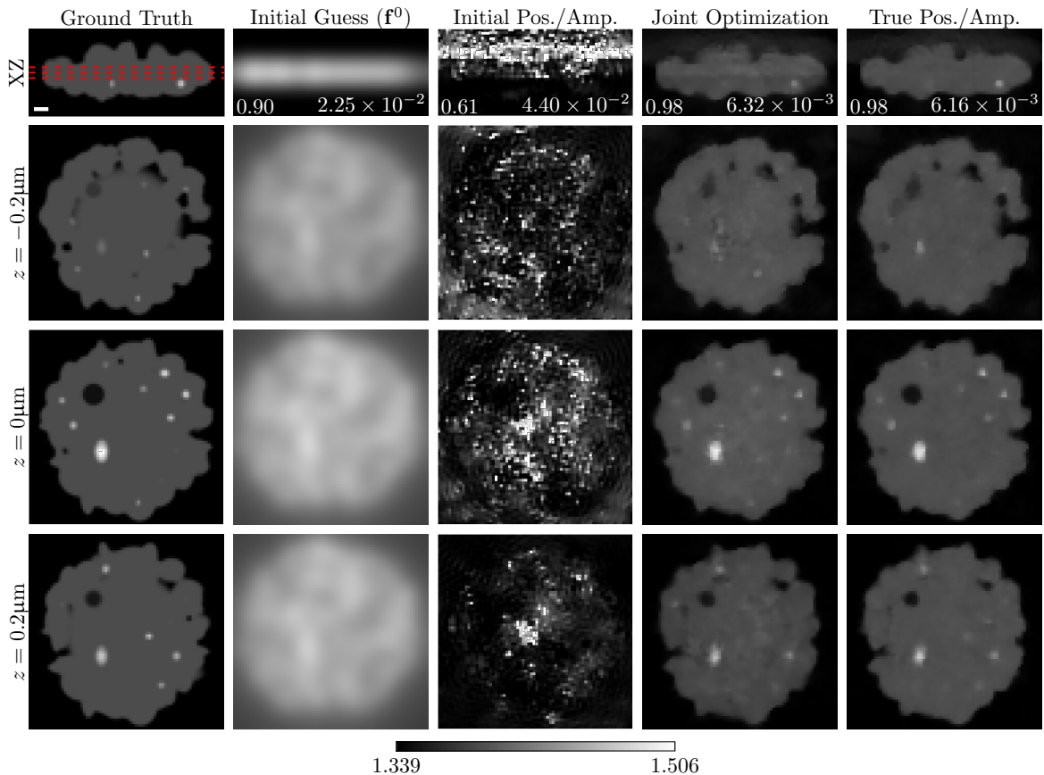
Figure 3: Reconstructions of the RI volume. From left to right: Ground truth, initial guess, reconstruction with positions and amplitudes fixed to their initial values (see Section 3.4.2), reconstruction with the proposed joint-optimization framework, and reconstruction with positions and amplitudes fixed to their true values (gold-standard). The SSIM and relative errors are displayed in the first row at the left and right corners, respectively, of each corresponding reconstruction. Scale bar: 500nm.
