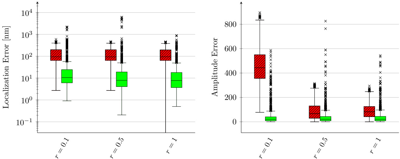
Figure 8: Box plots of the localization (left) and amplitude (right) error for different noise levels. Three noise levels are displayed with r = 0.1, 0.5, and 1 . For each case, the left box plot (hatched) corresponds to the initial positions/amplitudes and the right box plot (solid) corresponds to the refined positions/amplitudes. Note that the estimated amplitudes were scaled by r^{-1} to compare with the same ground-truth. For the box plots of the localization error after refinement (solid), we set the upper whiskers to 50\text{nm} so as to consider any larger error as outliers. This is in line with the expected 3D localization error in SMLM [6]. This bound is not relevant for the initial errors (hatched) as they are too large. For the hatched box plots, we thus set the default upper whiskers to Q3 + 1.5\text{IQR} , where \text{IQR} = (Q3 - Q1) is the interquartile range and Q1, Q3 are the 25th and 75th percentile, respectively. Finally, the lower whiskers are always set to the smallest error among all molecules. Outliers are indicated by \times .
