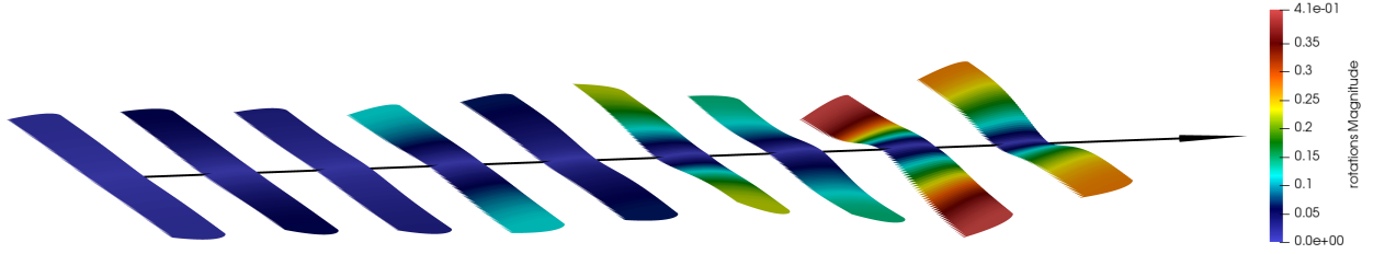
Figure 10: Real time flutter instability of the Patil wing; altitude = 20 km; velocity = 38 m/s
