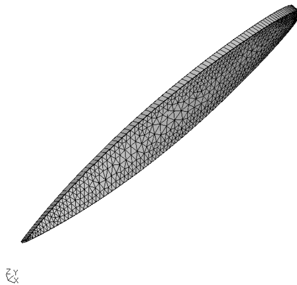
Figure 4: Warping of a NACA0015 airfoil section (amplified); CalculiX GraphiX
