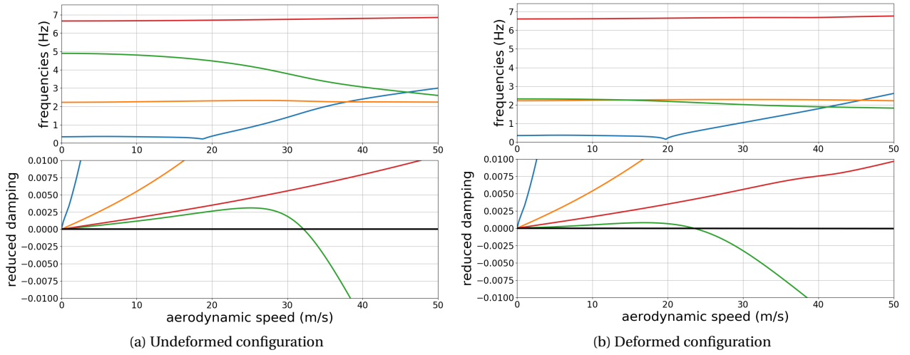
Figure 9: Patil wing aeroelastic modes
