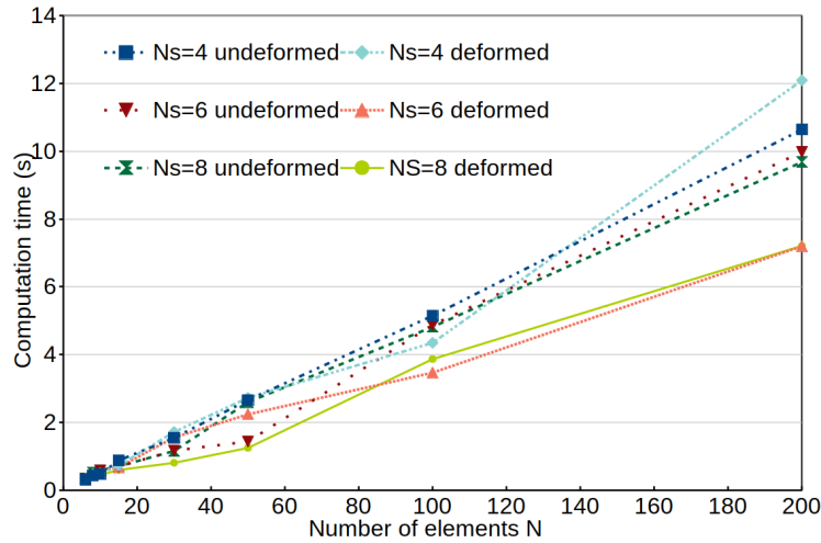
Figure 11: Patil flutter speed computation time (precision: 10^{-1} m/s)
