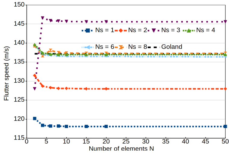
Figure 8: Convergence tests for N and N_s parameters for the Goland test case
