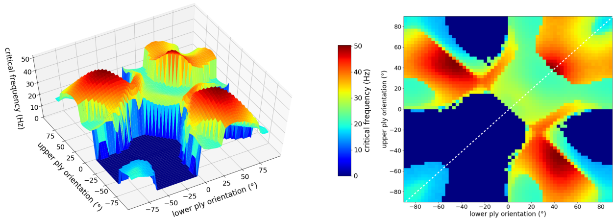
(c) Critical frequency
