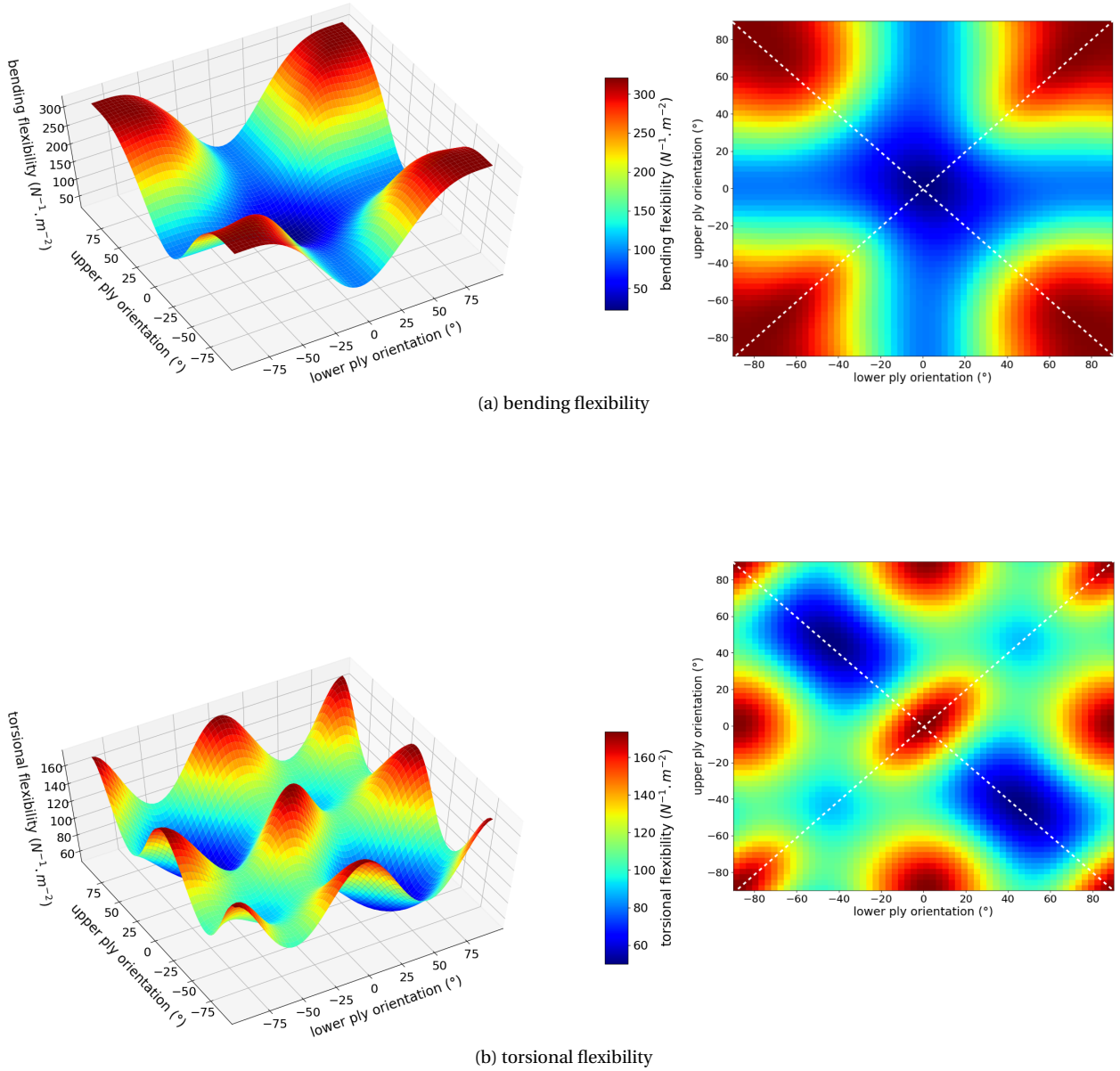
Figure 14: Composite laminates numerical simulation depending on lower and upper ply orientation : bending and torsional flexibility (symmetry axis in white dashed line)
