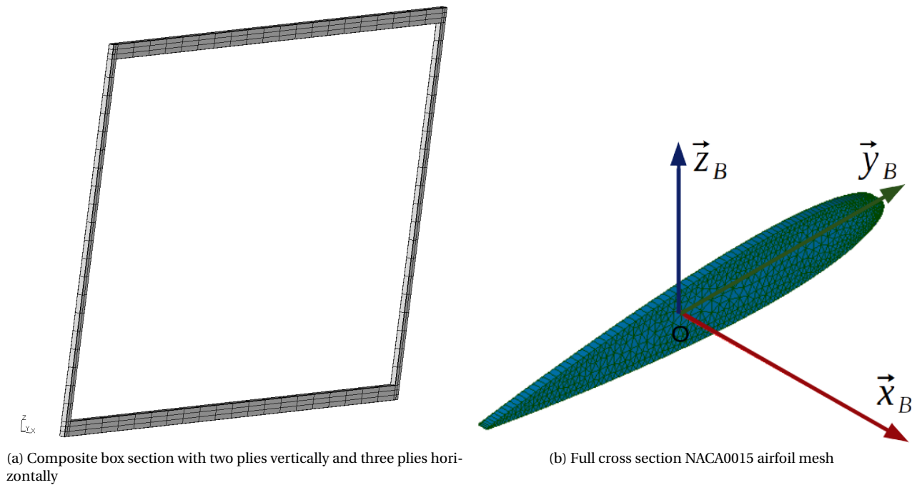
Figure 3: Examples of meshes used for the homogenisation
