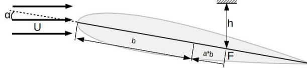
Figure 5: Airfoil parameters
