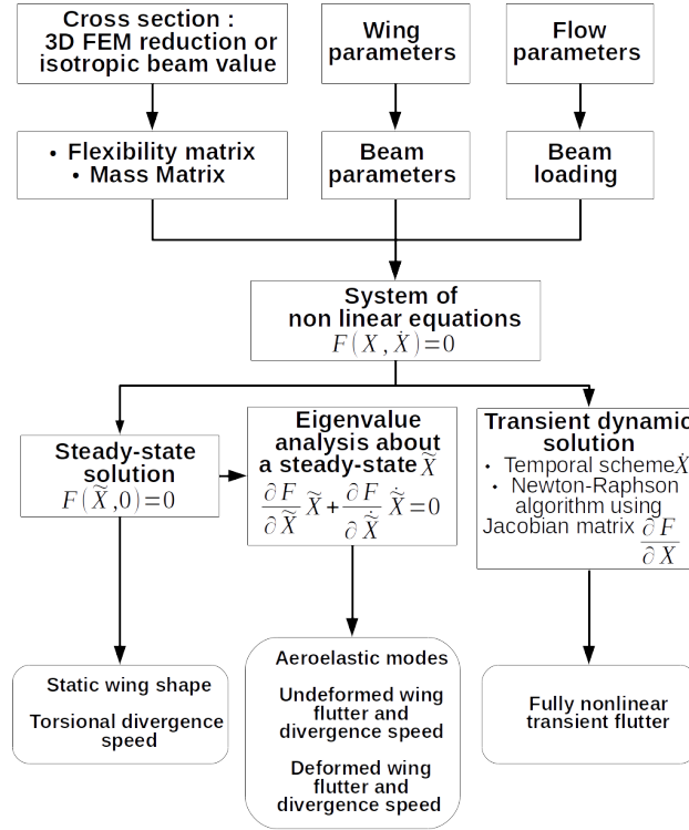
Figure 7: GEBTAero computation features
