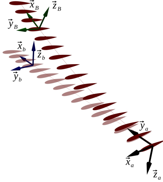
Figure 2: Structural frames definition
