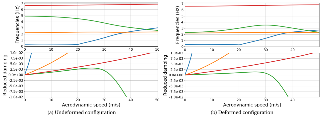
Figure 12: Anisotropic Patil wing aeroelastic modes plot
