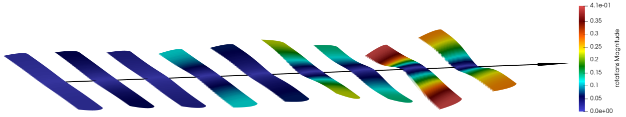
Figure 10: Real time flutter instability of the Patil wing; altitude = 20 km; velocity = 38 m/s
