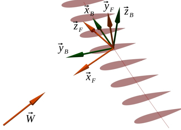
Figure 6: Flow frame definition
