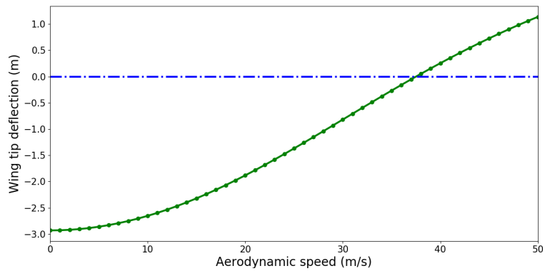
Figure 13: Anisotropic Patil wing static tip deflection depending on flow speed.
