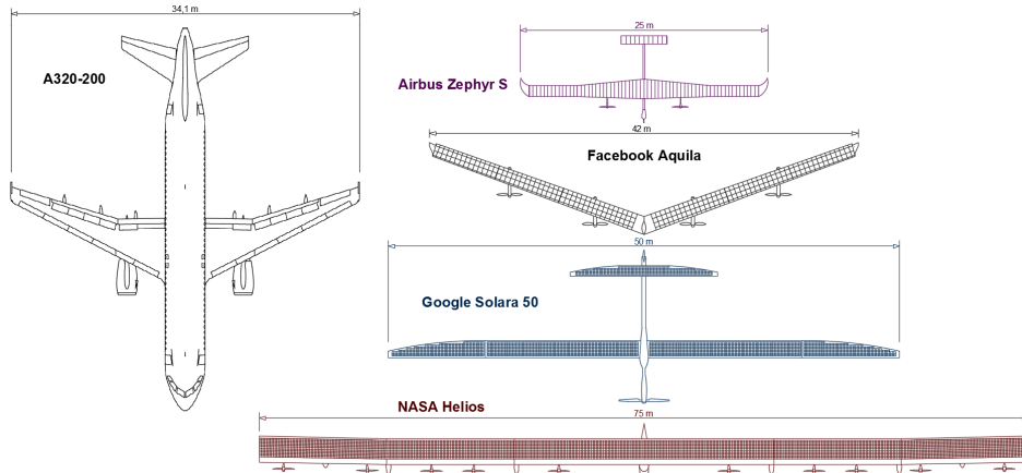
Figure 1: Sketch of some HAPS projects with a comparison against Airbus A320-200 dimensions
