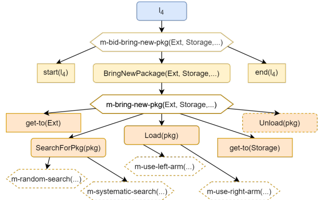
Figure 3: Illustration of the decomposition of labeled task l_4 for the bid estimation of the BorderDelivery problem. Hexagons represent methods, rounded rectangles represent compound tasks while sharp rectangles are primitive tasks, dotted lines represent nodes with hidden decompositions. Blue nodes represent elements from \mathcal{H} . The specific decomposition for the bid estimation is represented in yellow. Local decomposition nodes are represented in orange.
