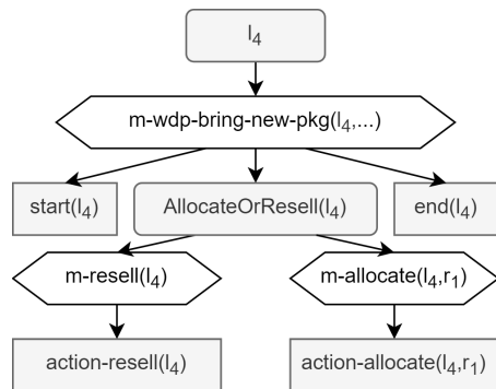
Figure 4: Decomposition of task l_4 integrating received bids for the WDP of the BorderDelivery problem. Hexagons represent methods, rounded rectangles represent compound task while sharp rectangles are primitive tasks.
