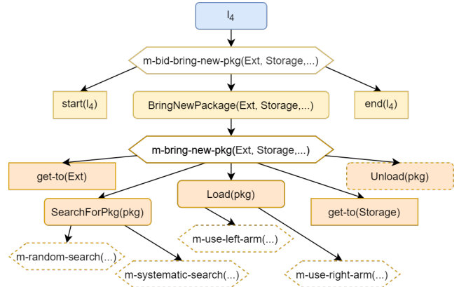
Figure 3: Illustration of the decomposition of labeled task l_4 for the bid estimation of the BorderDelivery problem. Hexagons represent methods, rounded rectangles represent compound tasks while sharp rectangles are primitive tasks, dotted lines represent nodes with hidden decompositions. Blue nodes represent elements from \mathcal{H} . The specific decomposition for the bid estimation is represented in yellow. Local decomposition nodes are represented in orange.
