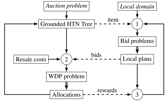
Figure 1: Protocol description. Rectangles represent information or data structures managed by the agents. Blocks on the left are managed by the auctioneer, blocks on the right by each bidder. Dashed arrows represent data exchanged between the auctioneer and the bidders. Circles indicate processes that aggregate information to build new structures. Double arrows indicate calls to a HTN planner.
