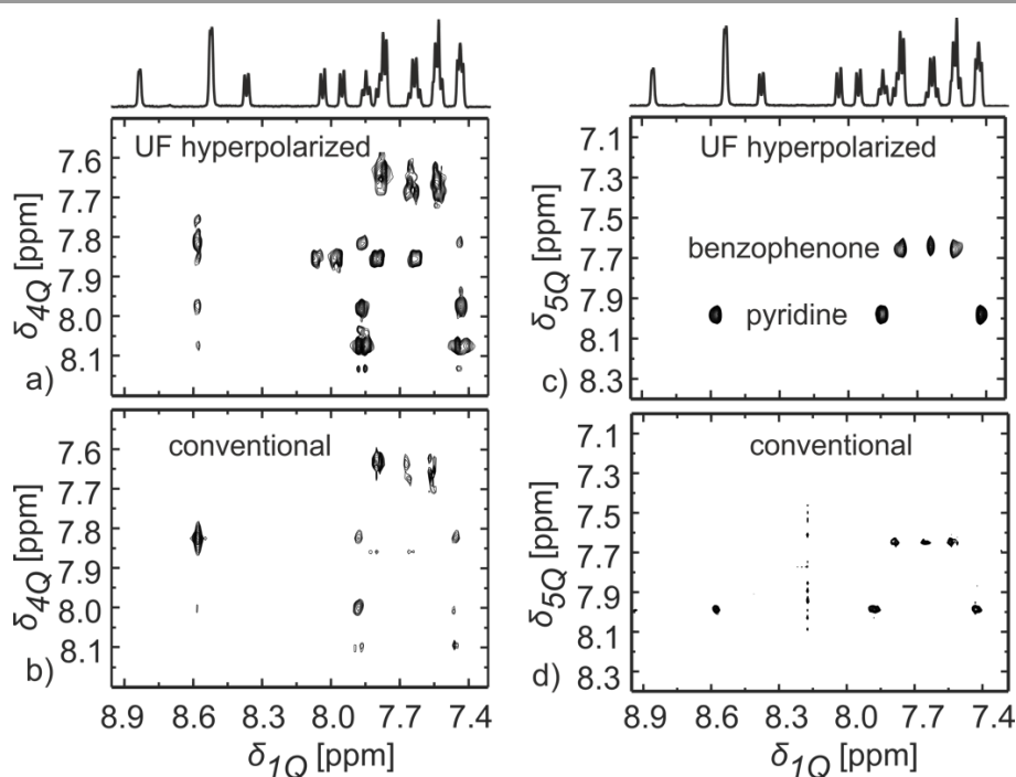
Figure 3 a) 2D ^1\text{H} - ^1\text{H} UF 4Q/1Q spectrum obtained in a single scan on a similar hyperpolarized mixture as described in Fig. 1d. b) Conventional 2D ^1\text{H} - ^1\text{H} 4Q/1Q spectrum measured on the same sample after rethermalisation and shimming in 8 hours and 3 minutes using 64 t_1 increment steps with 32 scans per increment. c) Same as a) but targeting a 2D ^1\text{H} - ^1\text{H} hyperpolarized 5Q/1Q NMR spectrum in a single scan. d) Same as b) but for a conventional 2D ^1\text{H} - ^1\text{H} 5Q/1Q spectrum measured on the same sample after rethermalisation and shimming in 8 hours and 3 minutes using 64 t_1 increment steps with 32 scans per increment. The data for obtaining the conventional spectra were processed with same acquisition ( t_2 ) and evolution ( t_1 ) times as used for its corresponding 2D hyperpolarized UF spectra. Shown on top of the 2D sets is the conventional 1D spectrum for this mixture.
