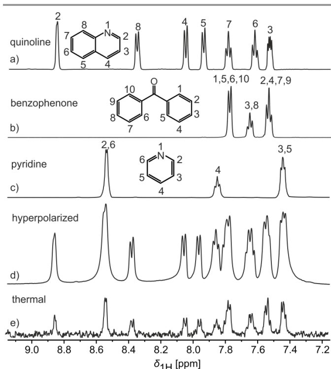
Figure 1 1D ^1\text{H} NMR spectra obtained for thermally-polarized a) quinoline (0.26 M); b) benzophenone (0.34 M); c) pyridine (0.38 M); d) a hyperpolarized mixture (85 mM) of pyridine, quinoline and benzophenone at 11.7 T obtained with a small flip angle ( \sim 1^\circ ); e) the same sample as d), post-dissolution, rethermalization and shimming, collected under the same acquisition conditions as d) in a single scan. Hyperpolarization was achieved after 45 minutes of irradiation at 94.150 GHz, of a glassy sample at 1.2–1.3 K.
