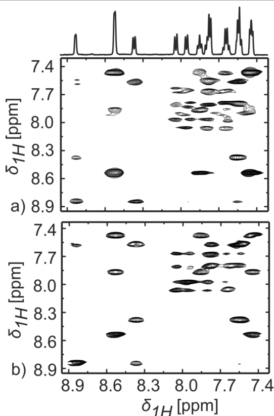
Figure 2 a) 2D ^1\text{H} - ^1\text{H} hyperpolarised UF TOCSY spectrum obtained in a single scan using this sequence on the sample described in Fig. 1d). b) Conventional 2D ^1\text{H} - ^1\text{H} TOCSY spectrum measured on the same sample after rethermalisation and shimming, in 4 hours and 25 minutes using 128 t_1 increments with 8 scans per increment. The data for obtaining the conventional spectra were processed with same acquisition ( t_2 ) and evolution ( t_1 ) times as used for its corresponding 2D hyperpolarized UF spectra. Shown on top of the 2D sets is the conventional 1D spectrum for this mixture
