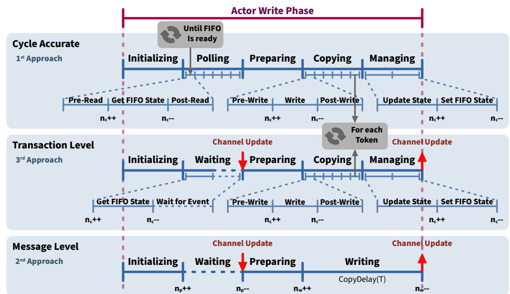
Figure 4. Simulation steps of the model of an actor write phase using two different communication models. cycle accurate [5] model at the top, message level [6] at the bottom and new transaction level model in the middle.
