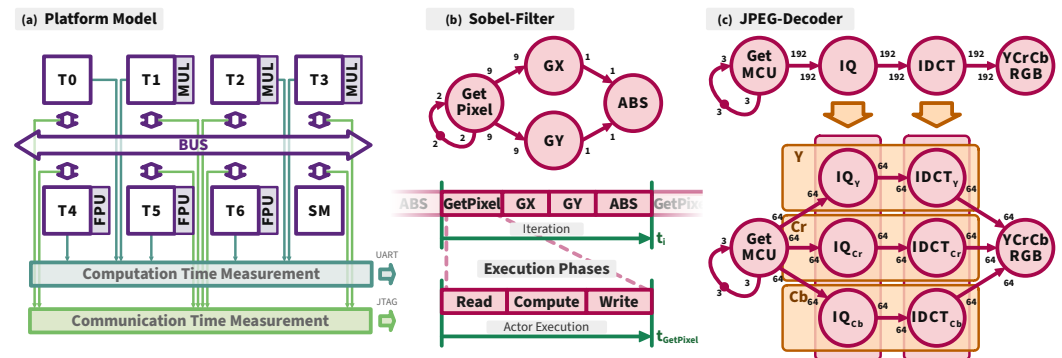
Figure 2. (a) Shows the architecture model of our evaluation platform (purple) and the measurement infrastructure (green) for characterization. (b) Shows details of the computation model on our Sobel-Filter Use-Case. (c) Shows our JPEG decoder Use-Case with and without considering data dependent behavior.
