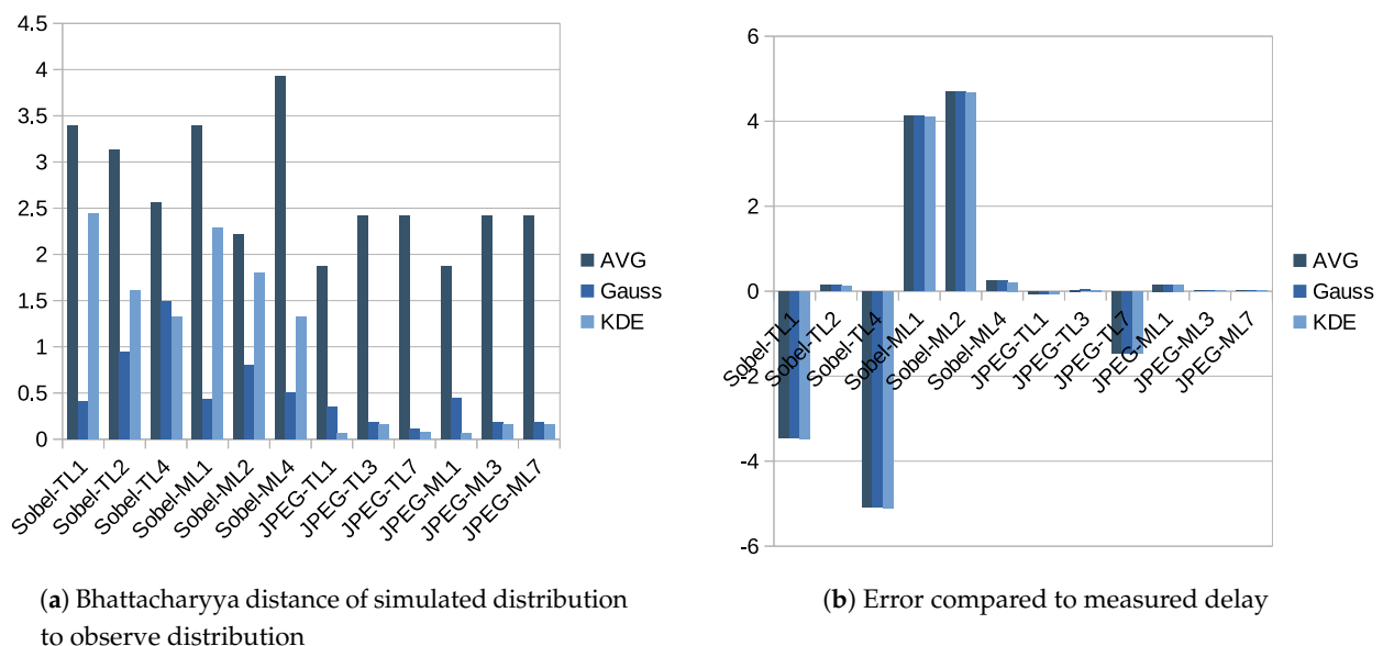
Figure 8. Comparison of the simulation results to the observed behavior of the Use-Cases on a real platform.
