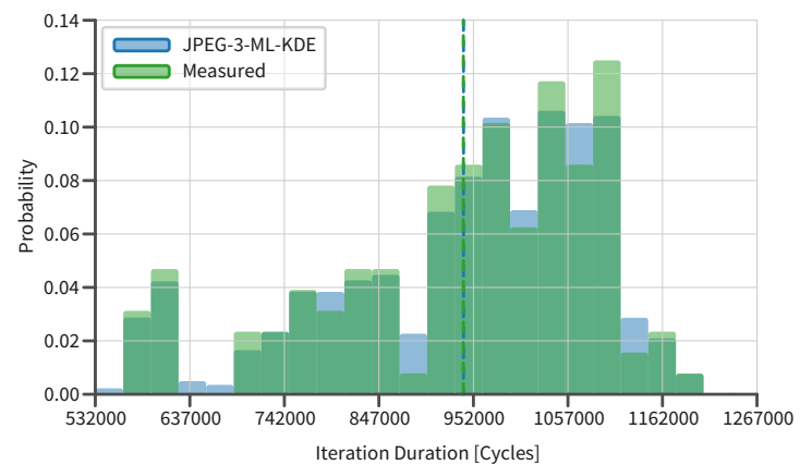
(d) JPEG Decoder on 3 Tiles (Realistic Mapping) using best communication and computation model.
