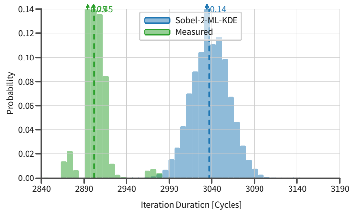
(c) Sobel on 2 Tiles (Realistic Mapping) using best communication and computation model.
