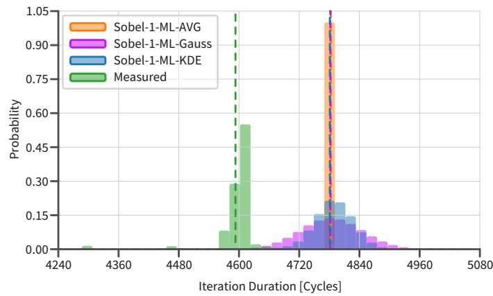
(a) Sobel on 1 Tile with ML communication model and different computation models compared to measured data
