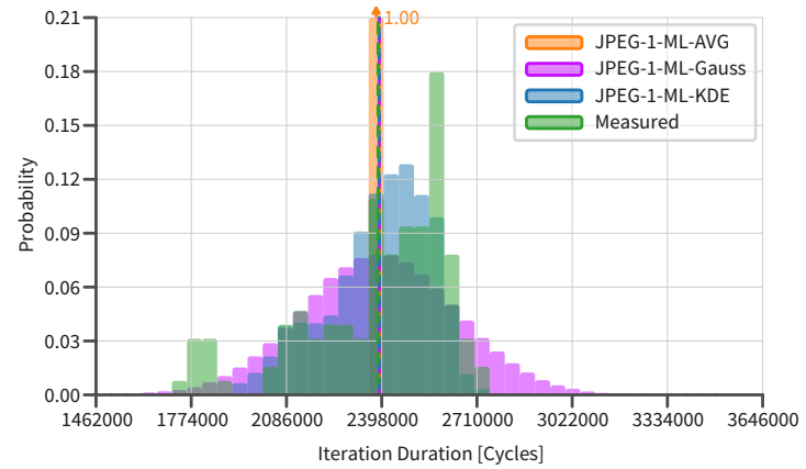
(b) JPEG Decoder on 1 Tile with ML communication model and different computation models compared to measured data
