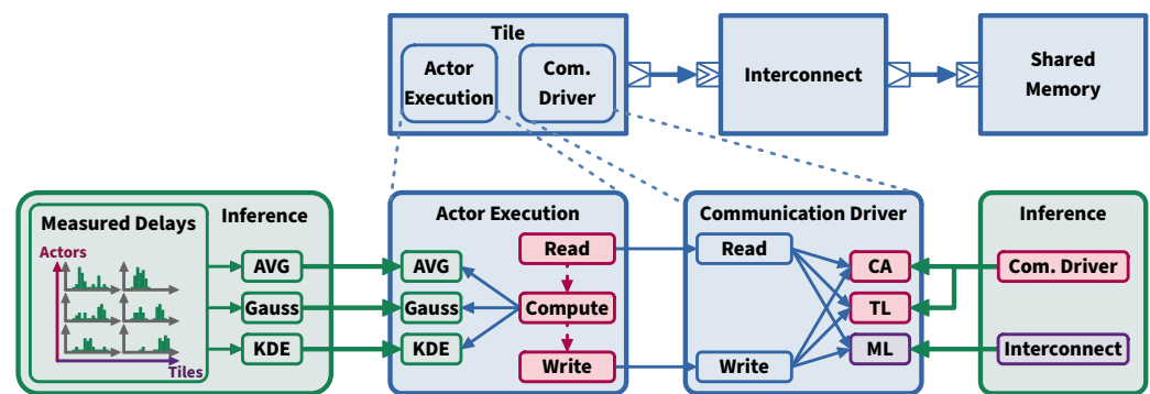
Figure 5. Architecture of our SystemC simulation showing how our models are integrated.
