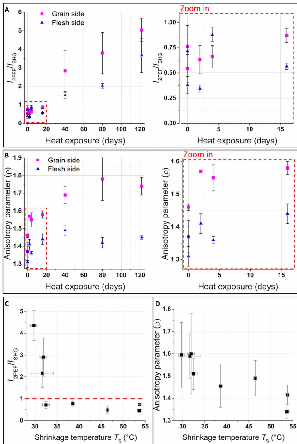
Fig. 3. Quantitative assessment of model parchments from NLO microscopy. (A) Ratio of 2PEF to SHG signals I_{2PEF}/I_{SHG} and (B) anisotropy parameter \rho on grain and flesh sides of the model parchments artificially aged by heat for 0, 2, 4, 16, 40, 80, and 122 days (one parchment for each treatment duration, but two reference parchments for D0). Zoom in (on the right): heat exposure for 0 to 16 days. (C) I_{2PEF}/I_{SHG} and (D) \rho mean values from both sides of the parchments versus the shrinkage temperature T_s determined by DSC. The red dashed line in (C) corresponds to I_{2PEF}/I_{SHG} = 1 . Error bars correspond to the SD of measurements on several samples ( T_s ) or several areas and sides ( I_{2PEF}/I_{SHG} , \rho ), depending on the technique (see table S1).
