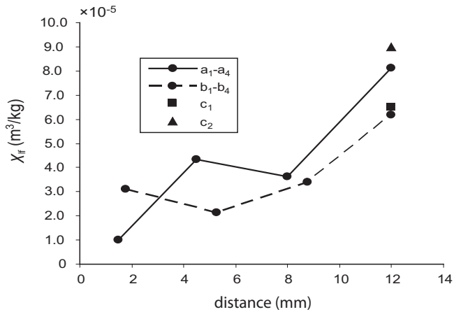
Fig. 8. Low-field magnetic susceptibility \chi_{lf} for subsamples of experimentally shocked Saratov meteorite (subsamples a_1 - a_4 correspond to A-shock experiment on a bulk Saratov sample and b_1 - b_4 correspond to B-shock experiment on a powdered Saratov sample) versus its distance from the center of the corresponding shocked spherical sample (every point corresponds approximately to the subsample center). \chi_{lf} values of the initial (experimentally unshocked) Saratov subsamples c_1 and c_2 are indicated by a square and a triangle.
