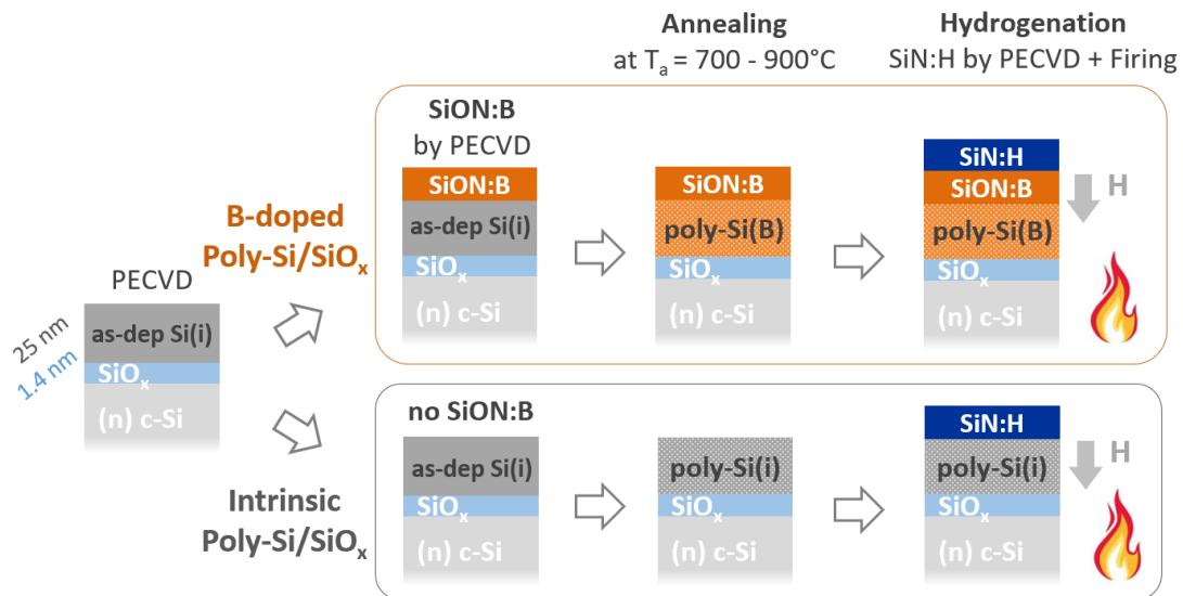
Figure 1. Schematic of the fabrication processes of B-doped and intrinsic poly-Si/SiO x contacts.
