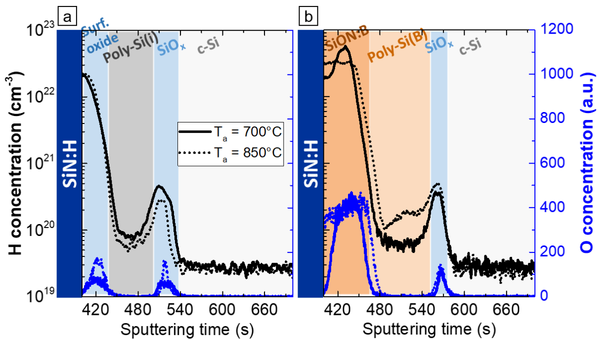
Figure 7. H and O concentration profiles (represented by black and blue lines, respectively) as measured by ToF-SIMS on samples featuring the poly-Si(i)/SiO x (a) and the poly-Si(B)/SiO x (b) contacts. Measurements were performed after SiN:H deposition on samples annealed at T_a = 700 °C (solid curves) and 850 °C (dashed curves).
