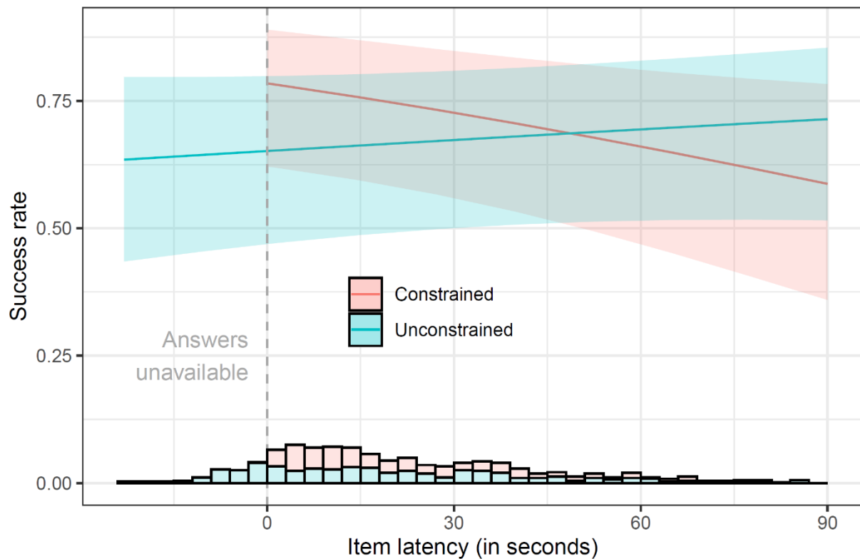
Figure 2. Success rate estimates from binomial mixed-effects model analysis in Experiment 2 as a function of condition and item latency. Item latencies were centered on imposed delay for each item, with no response possible before this delay in the Constrained condition. Histogram of item latencies overlaid at the bottom.
