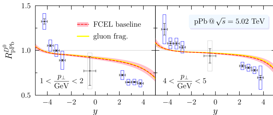
Figure 2. The rapidity dependence of R_{\text{pPb}}^{D^0} for D^0 production at \sqrt{s} = 5.02 TeV is shown for two p_{\perp} -bins. The baseline calculation is for the gg \rightarrow Q\bar{Q} channel in the center of each bin, compared with ALICE and LHCb data [47, 48]. (The curves labelled ‘gluon frag.’ correspond to the channel gg \rightarrow gG \rightarrow gQ\bar{Q} discussed in section 3.3.)
