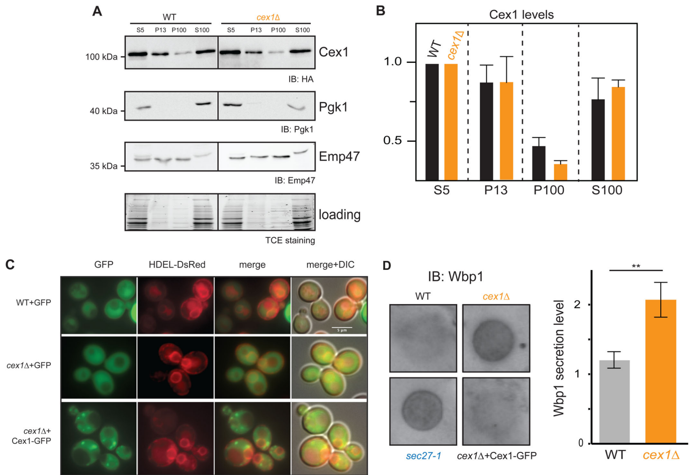
Fig. 4. Cex1 is associated to membrane fractions, and its deletion leads to defective trafficking of Wbp1, an ER protein having a di-lysine COPI sorting signal. (A) Subcellular fractionation of WT (SEY6210) and cex1Δ mutant strain, expressing the Cex1-HA fusion protein. Immunodetection of Cex1-HA in each fraction was done using anti-HA antibodies. Presence of cytosolic proteins in the different fraction was assessed by detecting the soluble Pgk1 protein, and ER as well as ER-Golgi vesicles resident protein by the integral membrane protein Emp47. Protein loading was controlled by TCE staining. (B) Cex1 protein levels detected in the P13, P100 and S100 fractions in A were measured using the total lysate (S5) as standard for each strain. Three independent replicates ( n=3 ) were used. Standard deviation is shown. Statistical analyses using the t -test was done; ** P<0.01 ; *** P<0.001 . (C) Intracellular localization of the HDEL-DsRED reporter localized at the ER via COPI trafficking was assessed by fluorescence microscopy. Scale bar: 5 \mu m. Representative micrographs are shown from analyses done on independent clones. (D) Trafficking of Wbp1, an effector of N-glycosylation bearing a KK COPI retrieval motif, was assessed by a dot-blot assay on WT, sec27-1 , cex1Δ and cex1Δ +Cex1-GFP cells grown in fermentation conditions (SC medium, at 25°C). Statistical analysis from data obtained from three independent clones was done using the t -test; ** P=0.01 .
