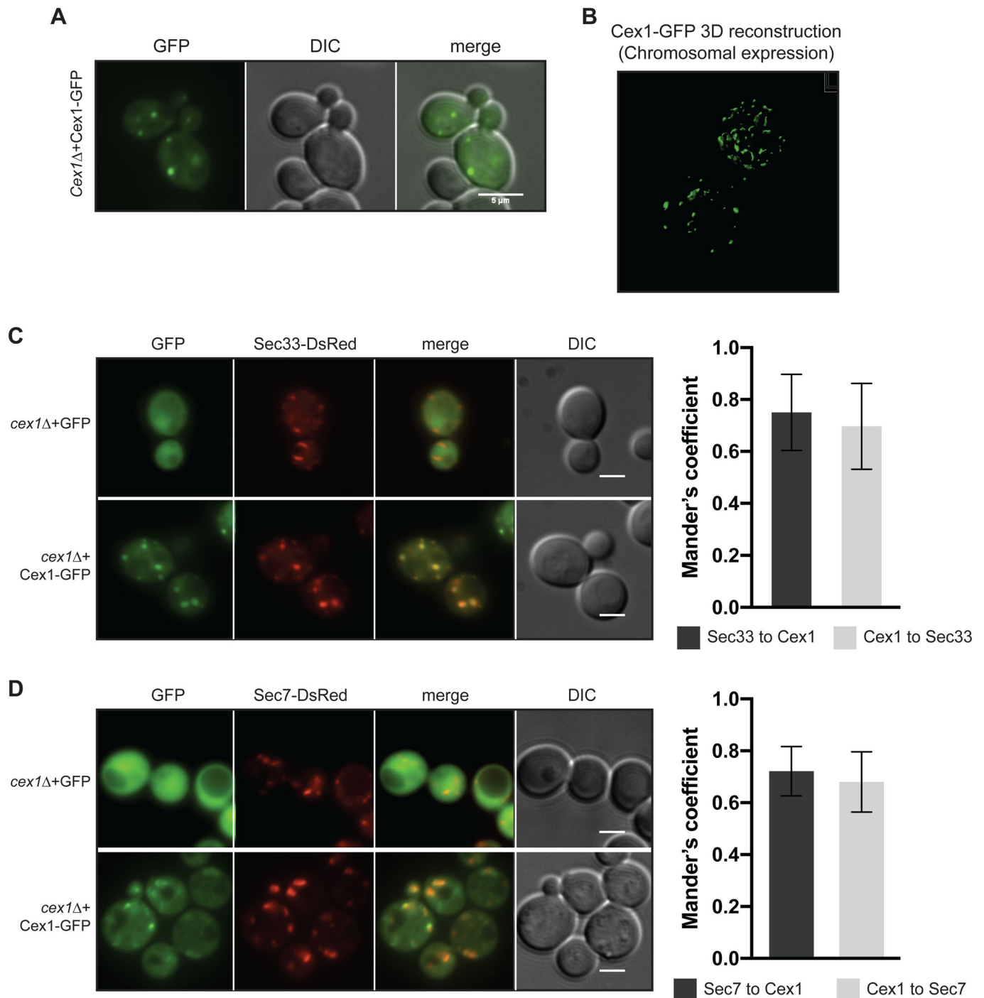
Fig. 3. Cex1-GFP colocalizes with the \alpha -COP Sec33-DsRED. (A) Epifluorescence microscopy of Cex1-GFP expressed in a cex1Δ strain. (B) 3D reconstitution of the Cex1-GFP construct when expressed at its genomic locus. (C) The Sec33 (Cop1/Ret1) COPI component was tagged with DsRED and its intracellular localization analyzed upon Cex1-GFP expression. cex1Δ cells expressing GFP alone were used as control. The colocalization of both markers were measured by Mander's coefficient (right panel). (D) Sec7-DsRED was used as a trans -Golgi marker together with Cex1-GFP. Their colocalization was measured by Mander's coefficient (right panel). cex1Δ cells expressing GFP alone were used as control. Scale bars: 5 μm. Representative micrographs from analyses done on different independent clones are shown.
