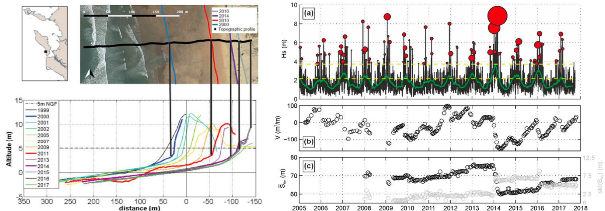
Fig. 2. Time-series using the datasets of Oléron and Truc Vert beaches. Decadal shoreline changes at Saint Trojan beach (Oléron) identified using shoreline mapping (top left) and topographic profiles (bottom left). (Right) (a) 3-hourly H_s (black) and 2-month moving average of H_s (thick green) using wave hindcast data. Red bubbles are storm events ( H_s > H_{s95\%} ), whereby the size of the bubbles is proportional to storm duration. Beach-dune volume above mean sea level (b), and mean (black) and longshore standard deviation (grey) of the 6-m elevation shoreline (c), determined using topographic quad-mounted GNSS DEM surveys. Adapted from Castelle et al. (2019) and Chaumillon et al. (2019).
