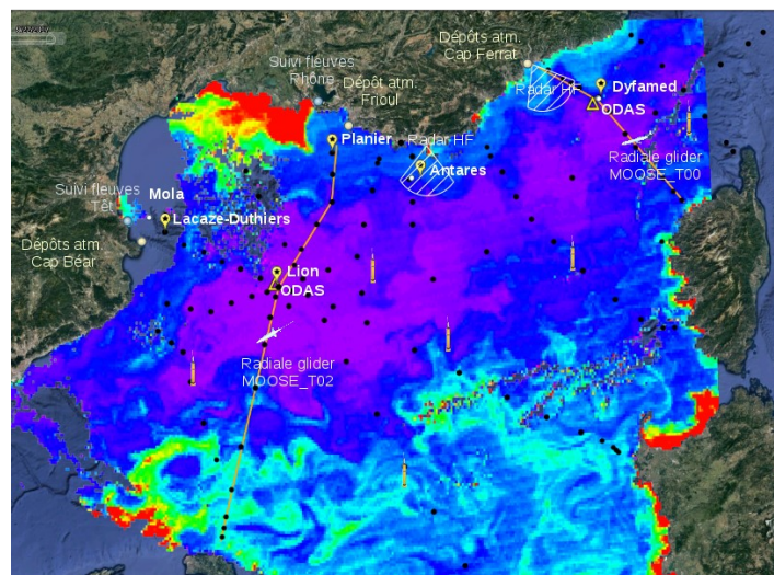
Fig. 1. Surface chlorophyll-a observed by satellite in February 2013 during a deep convection event (the dilution of phytoplankton is visible in purple). The MOOSE network : rivers and atmospheric deposit time series (blue/white dots on land), high-frequency radars (barred area), fixed mooring sites (yellow pins), surface meteorological buoys (ODAS triangles), autonomous platforms (endurance glider lines in orange, profiling floats drifting with currents) and ship-board surveys (black dots : yearly basin-scale cruise; white dots : monthly stations). LION, ANTARES & DYFAMED moorings are integrated in EMSO ERIC.
