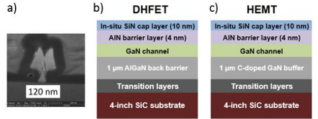
Fig. 1. a) FIB view of the 0.12 \mu m T-gate and schematic cross section of b) DHFET and c) C-doped HEMT.
