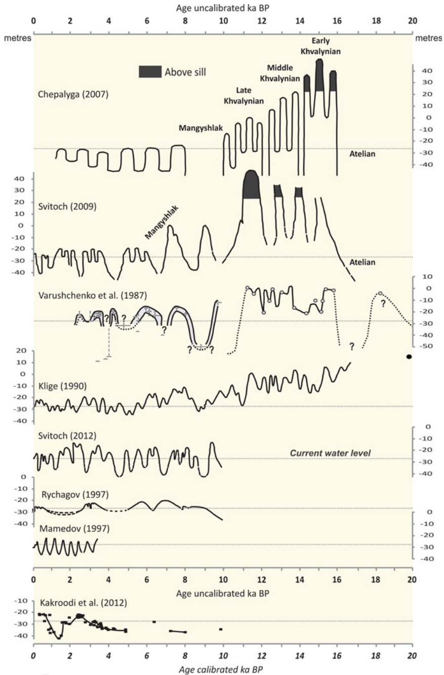
Fig. 3.5 Different Caspian Sea level reconstructions since the Last Glacial Maximum. In black, water levels above the sill flowing to the Black Sea (upper two panels)
