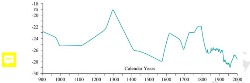
Fig. 3.6 Caspian Sea level curve based on historical data and instrumental measurements modified from Naderi Beni et al. (2013)
