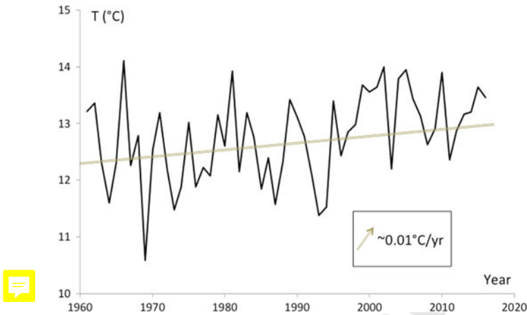
Fig. 3.8 Sea Surface Temperature at the station of Makhshkala in Russia on the western coast of the CS. Data from in situ gauge over the period from 1960 to 2016. The arrow shows the 0.01 °C increase per year. Source http://www.caspcom.com
