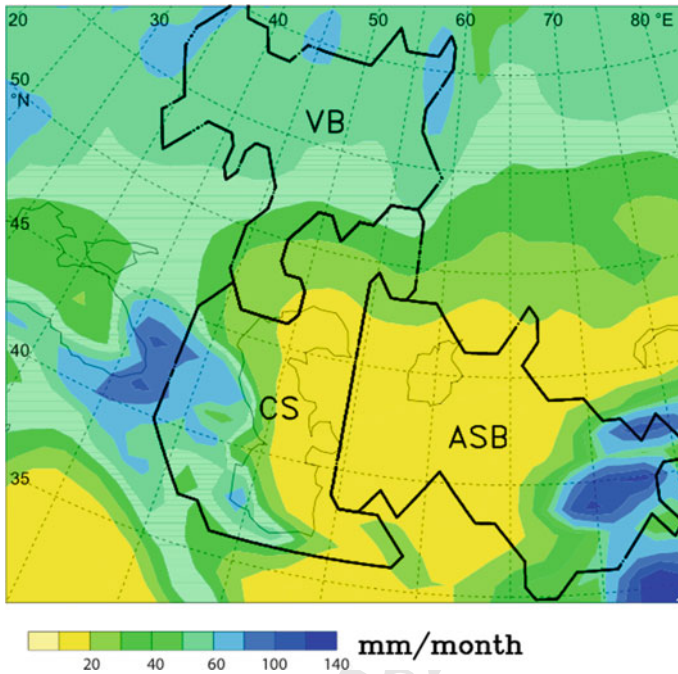
Fig. 3.3 Precipitations in mm per month (colour scale) and drainage basins (bold black line) over the Volga (VB) and the Amu-Darya and Syr-Darya (ASB) basins (provided graciously by K. Arpe)
