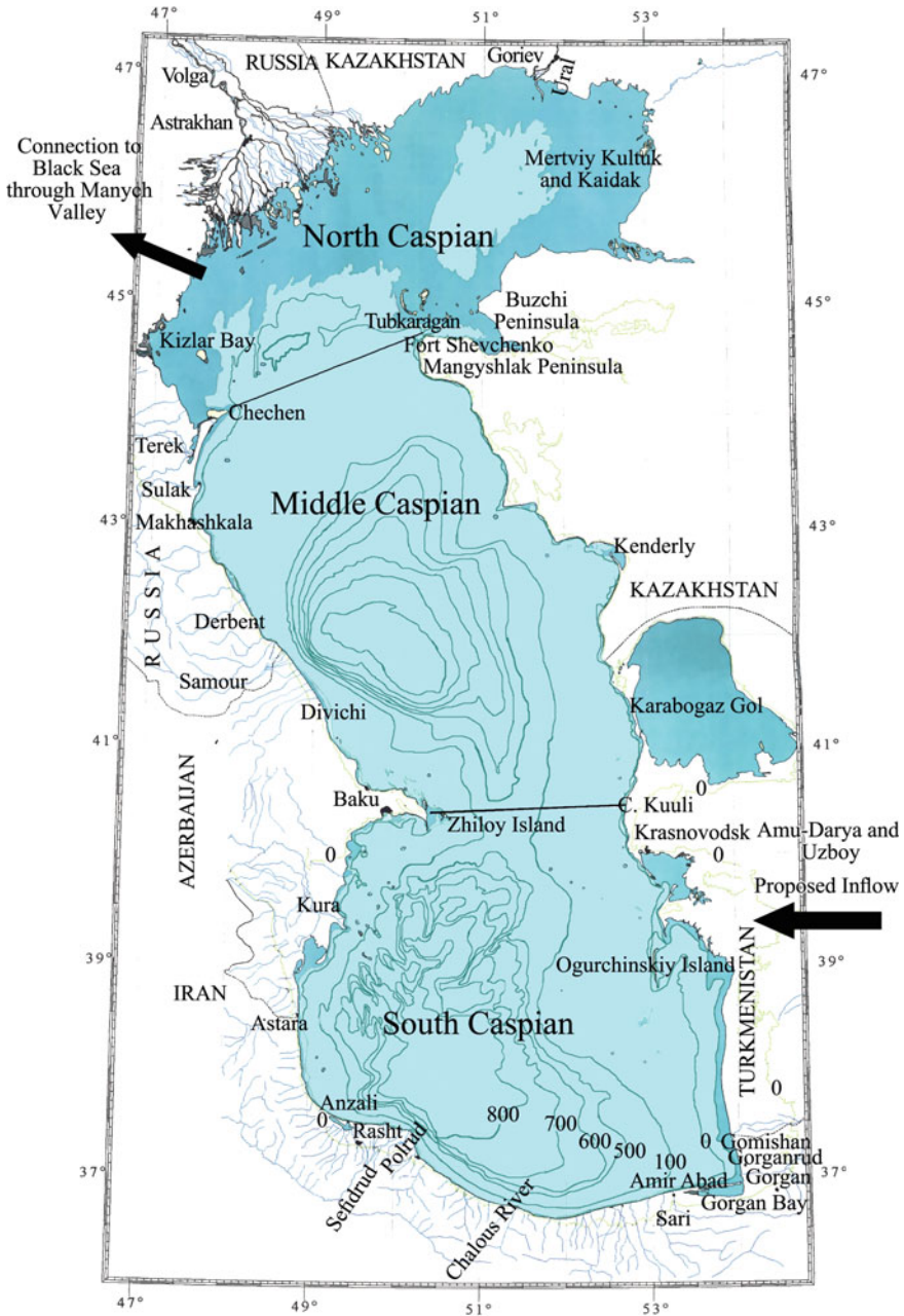
Fig. 3.1 Location map with bathymetry. The black lines through the Caspian Sea show the limit between its three basins. The green contour is the zero in the Baltic datum
