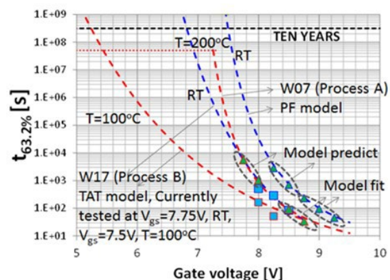
Figure 5: Operating lifetime prediction under forward bias condition at RT and 200°C based on thermally assisted tunneling and Poole-Frenkel model. Measured data (blue squares) are in line with the predicted lifetime models.
