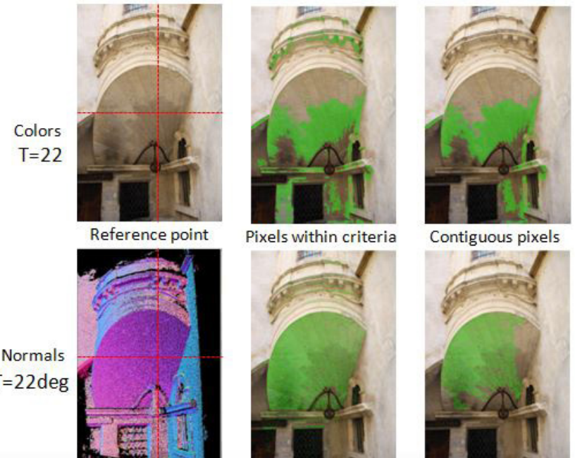
Fig. 14 - The transcription of the 3D magic wand tool can be very useful for the annotation of architectural elements, whose paths often follow simple geometric primitives. Here, the normals allow to quickly select planes, and to reproject them in 2D on the project images.
