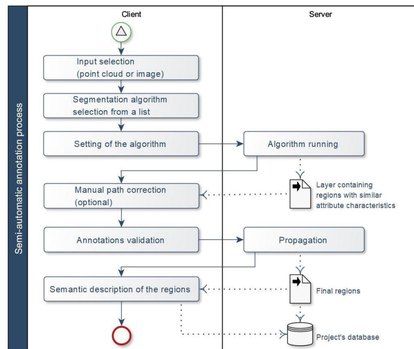
Fig. 15 - Semi-automatic annotation process based on segmentation algorithms.
