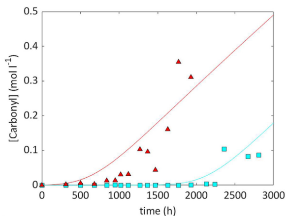
Fig. 6. Kinetic modeling of carbonyl build up at 80°C under air as for hypothesis 1: various initial concentration in unstable groups: [POOH]_0 = 0.0001 and 0.15 \text{ mol l}^{-1} for red and blue curve, respectively.
