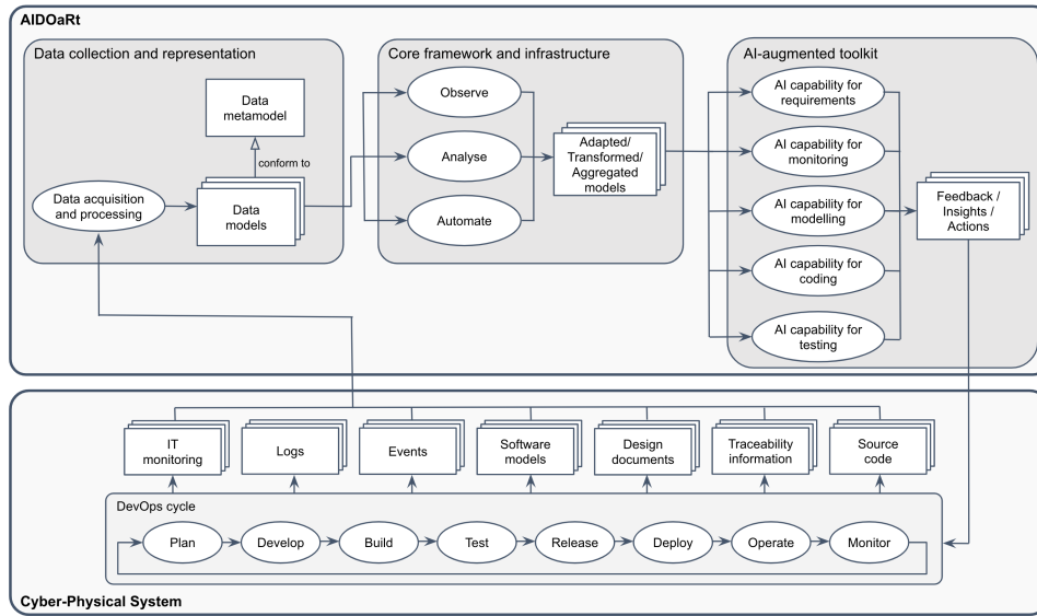
Figure 2. AIDOaRt Approach.
