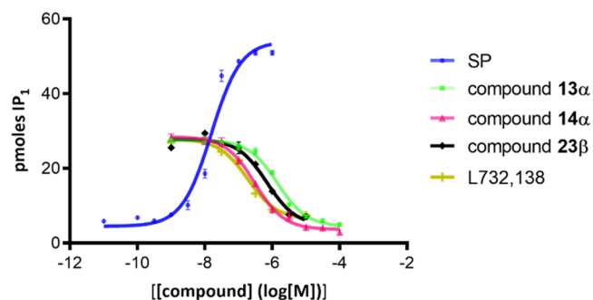
Figure 4. Concentration–response curves for the agonist and antagonist effects of SP (blue), L732,138 (olive green), \alpha -D-galactosyl derivatives ( 13 \alpha green; 14 \alpha pink), and \beta -D-arabinosyl derivative 23 \beta (black) using the IPone assay. The IP 1 accumulation (pmoles) was measured as described in the Experimental Section. Data are illustrated from a representative experiment performed at least three times.
