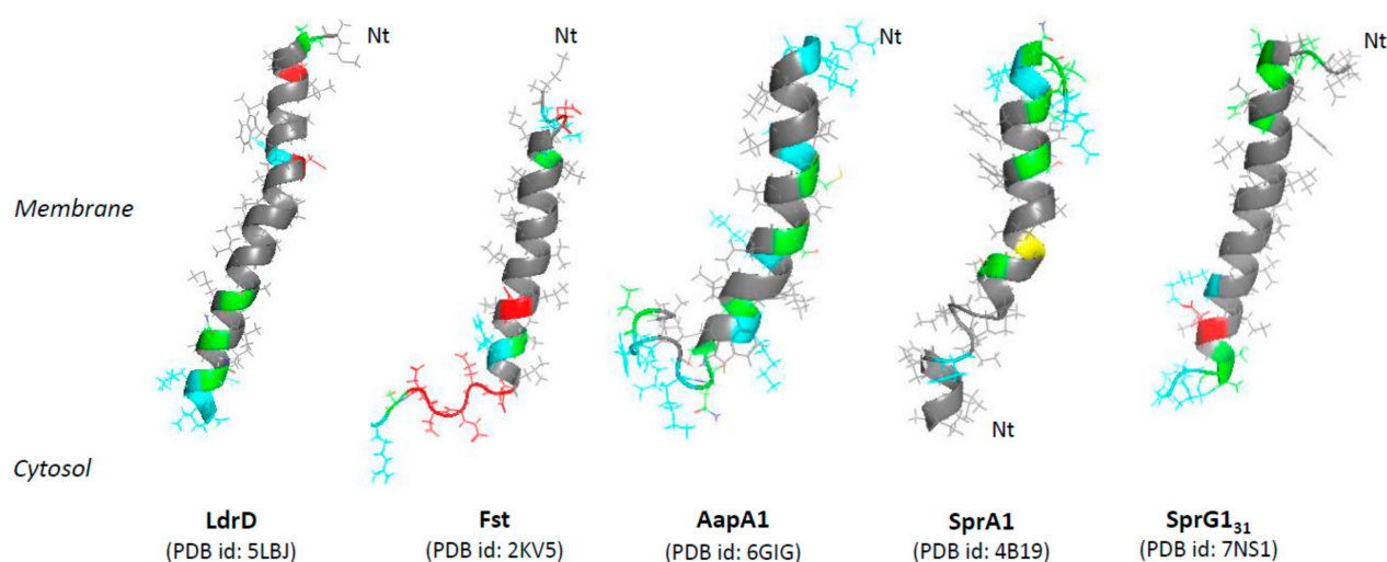
Figure 1. Overview of the structurally determined membrane-associated type I toxins. Hydrophobic amino acids are represented in gray, polar amino acids in green, positively charged amino acids in blue, negatively charged amino acids in red, and cysteines in yellow.
