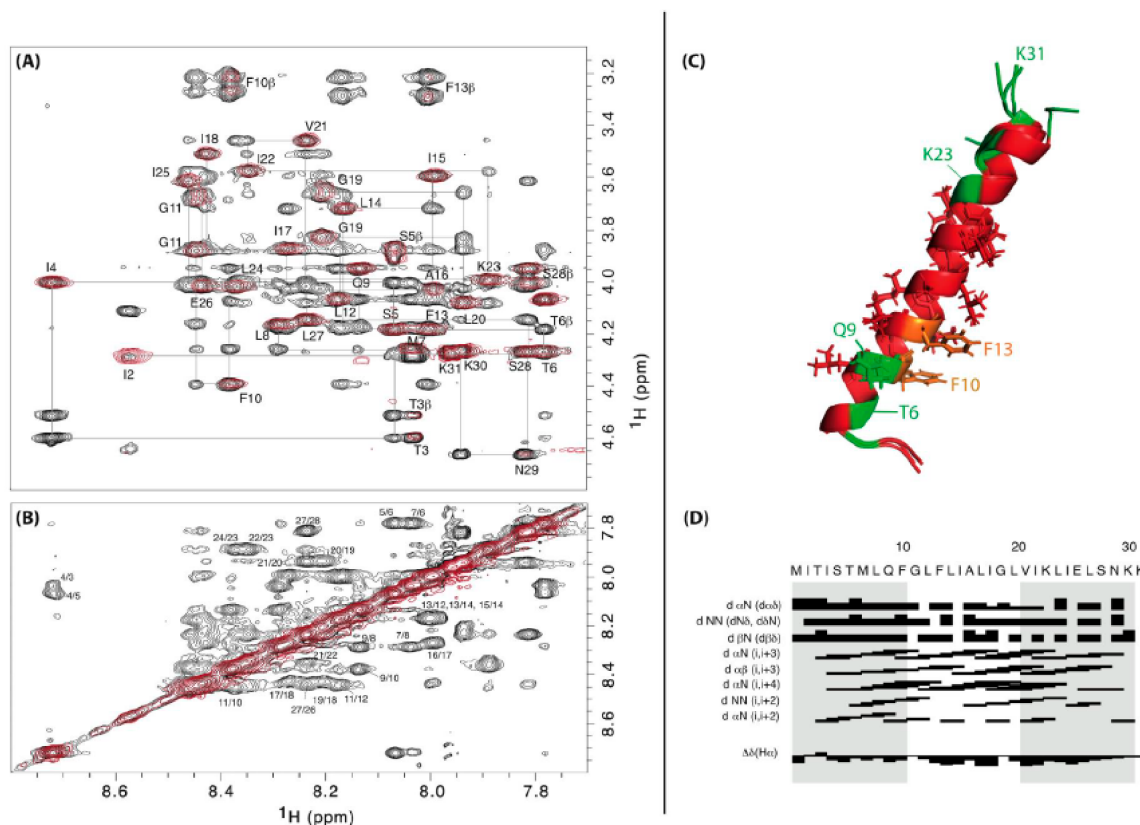
Figure 4. New SprG1 31 NMR 3D model of structure (PDB 7NS1). (A,B) Superposition of the 300 ms ^1\text{H} - ^1\text{H} NOESY spectrum (black) and the 80 ms ^1\text{H} - ^1\text{H} TOCSY spectra (red), both recorded at 303K and pH 4.5, showing the NH-H \alpha (panel A) and NH-NH (panel B) connectivities. (C) Superposition of the five best structures of lower energies and Molprobit scores: hydrophilic amino acids are in green, hydrophobic in red and phenylalanines in orange. (D) Distance restraints chart.
