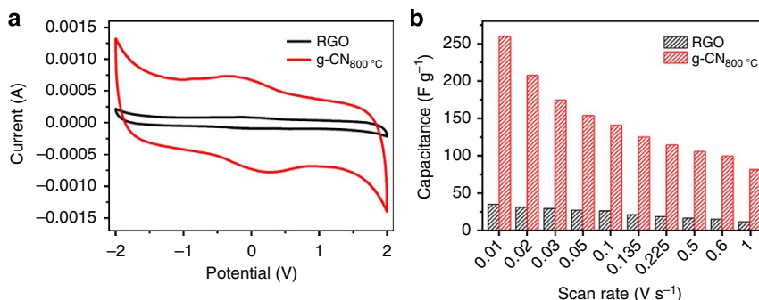
Figure 3 | Charge storage behaviour of the electrochemical actuators. (a) Cyclic voltammetry (CV) curves for the g-CN 800 °C and RGO electrode-based actuators at 10 \text{ mV s}^{-1} sweep rate. (b) The calculated capacitances of devices at different scan rates.
