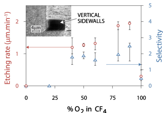
FIG. 3. (Color online) Etching rate at 300 W and 200 mTorr of microactuator precursor (O) and selectivity ( \Delta ) vs percent of \text{O}_2 in \text{CF}_4 . An optimal ratio of 90/10 was found with selectivity of 2.5 (IPN etch rate/photoresist etch rate). In inset, the vertical sidewalls obtained after etching at 90/10.
