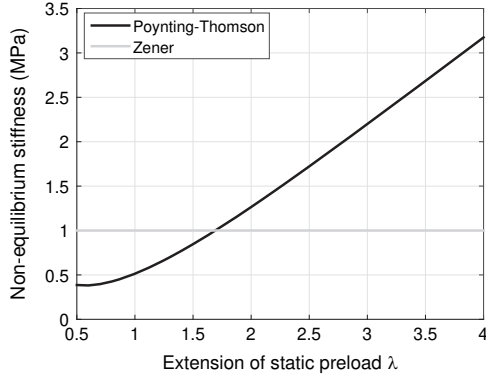
Fig. 4. Evolution of out-of-equilibrium stiffness during infinitely fast oscillations with respect to extension of a static preload, predicted by Zener and Poynting-Thomson models with C_1=0.3 MPa, C_2=0.75 MPa and C_{b2}=2 MPa.
