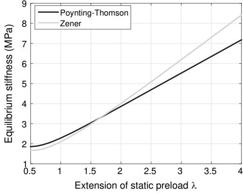
Fig. 3. Evolution of equilibrium stiffness with respect to extension of a static preload, predicted by Zener and Poynting–Thomson models with C_1=0.3 MPa, C_2=0.75 MPa and C_a=0.7 MPa.
