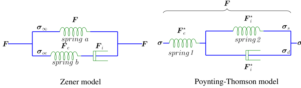
Fig. 1. Notations used in the Zener model and the Poynting–Thomson model for large strain formulation.
