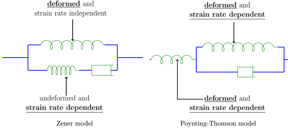
Fig. 2. Comparison of the state of each element in rheological schemes of Zener and Poynting–Thomson models after a static deformation.
