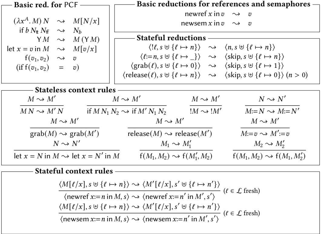
Fig. 24. Operational semantics of IPA
