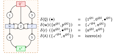
Fig. 6. Closed Petri structure for \text{coin} : \mathbb{B}
