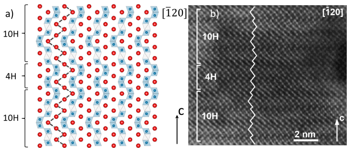
Figure 5: a) Representation of the stacking faults, in the 10\text{H-Ba}_5\text{Ru}_4\text{O}_{15} seen from the [-120] direction, Ba atoms are in red and \text{RuO}_6 octahedra are in blue. The black dotted line shows the sequence of \text{BaO}_3 layer. b) [-120] HAADF-STEM image
