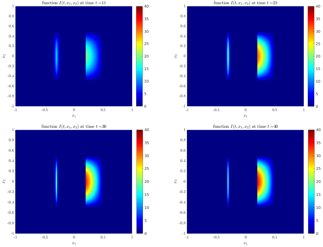
Figure 3: Illustration of Theorem 2.2 in the case i), i.e. , when I_0(\alpha^{-1}(\alpha^*)) > 0 . Function x \rightarrow I(t, x) at time t = 10, 20, 30 and 40 . The function I remains bounded in this case.
