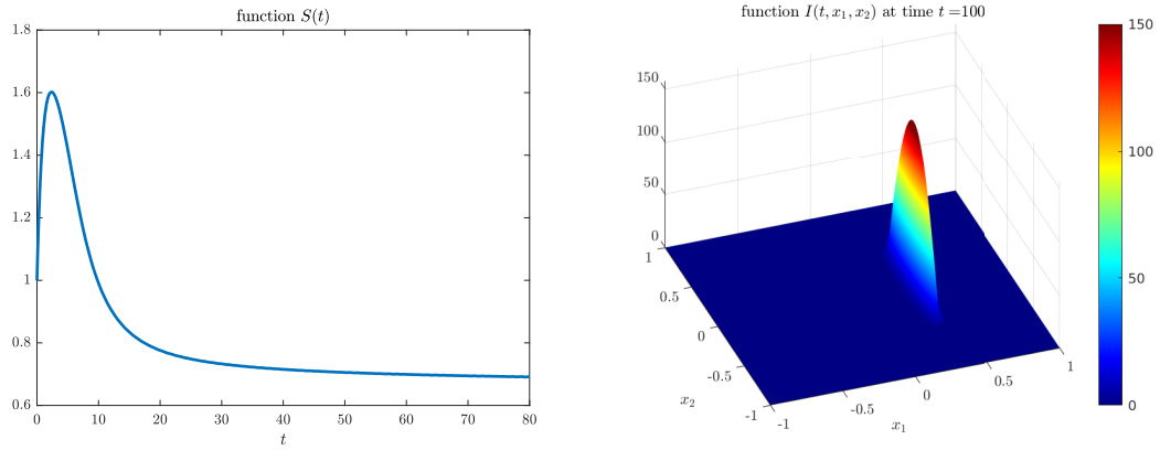
Figure 5: (continued from Fig. 4) Illustration of Theorem 2.2 in the case ii), i.e. when I_0(\alpha^{-1}(\alpha^*)) = 0 . Function t \rightarrow S(t) converges towards 1/\alpha^* = 2/3 . Function x \rightarrow I(t, x) at time t = 100 is asymptotically concentrated on \alpha^{-1}(\alpha^*) = \{0.35\} \times [-0.5, 0.5] .
