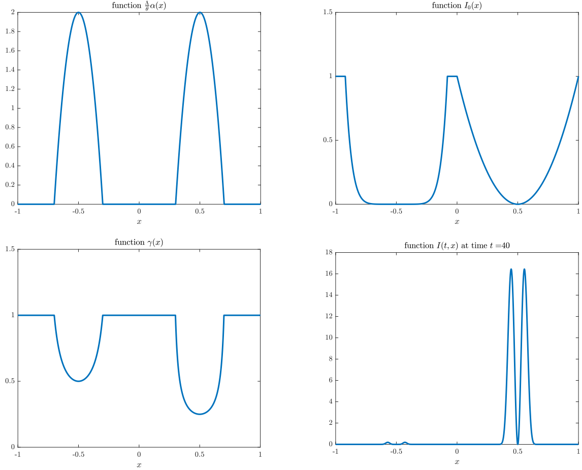
Figure 7: Illustration of Theorem 2.13 and Corollary 2.14. Parameters of this simulation are: \Lambda = 2 , \theta = 1 , \alpha(x) is given by (22), I_0(x) by (23) and \gamma(x) by (24). In particular, \alpha^* = 1 , \alpha^{-1}(\alpha^*) = \{x_1, x_2\} with x_1 = -0.5 , x_2 = 0.5 , \kappa_1 = 8 , \kappa_2 = 2 , \gamma(x_1) = 1/2 , \gamma(x_2) = 1/4 , \rho = 6 and J = \{2\} . The initial condition I_0 vanishes more rapidly around x_1 than x_2 so that the solution I(t, x) vanishes around x_1 as t goes to \infty , even though \gamma(x_1) > \gamma(x_2) , while around x_2 it takes the shape given by expression (2.14).
