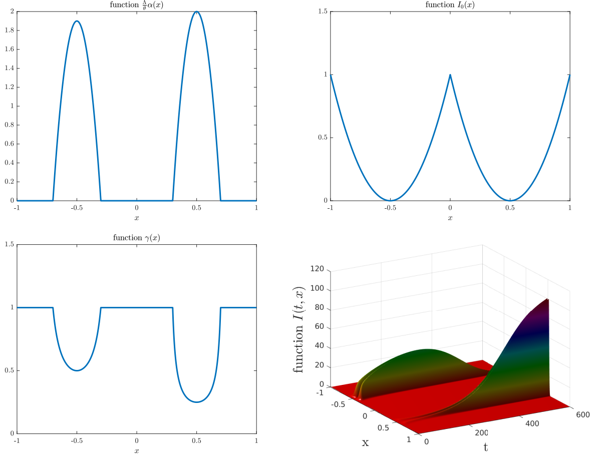
Figure 8: Illustration of a transient behavior for (1). Parameters of this simulation are: \Lambda = 2 , \theta = 1 , \alpha(x) is given by (25), I_0(x) by (26) and \gamma(x) by (27). In particular, \alpha^* = 1 , \alpha^{-1}(\alpha^*) = \{x_2\} with x_1 = -0.5 , x_2 = 0.5 . Other parameters are \kappa_1 = 2 , \kappa_2 = 2 , \gamma(x_1) = 1/2 , \gamma(x_2) = 1/4 . The value of the local maximum at x_1 , \alpha(x_1) = 0.95 , being very close to \alpha^* , observe that the distribution I(t, x) first concentrates around x_1 before the global maximum x_2 becomes dominant (bottom right plot).
