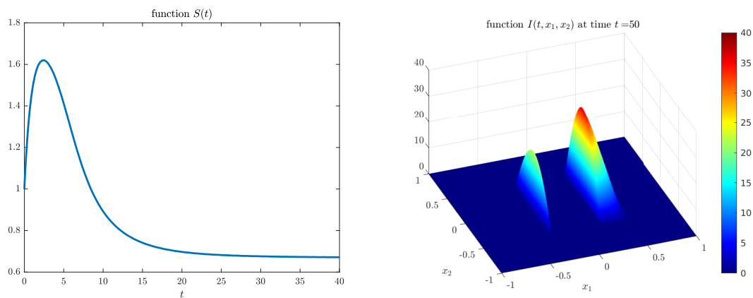
Figure 2: (continued from Fig. 1) Illustration of Theorem 2.2 in the case i), i.e. , when I_0(\alpha^{-1}(\alpha^*)) > 0 . Function t \rightarrow S(t) converges towards 1/\alpha^* = 2/3 and function x \rightarrow I(t, x) at time t = 50 is asymptotically concentrated on \alpha^{-1}(\alpha^*) = (\{-0.3\} \cup [0.2, 0.5]) \times [-0.5, 0.5] .
