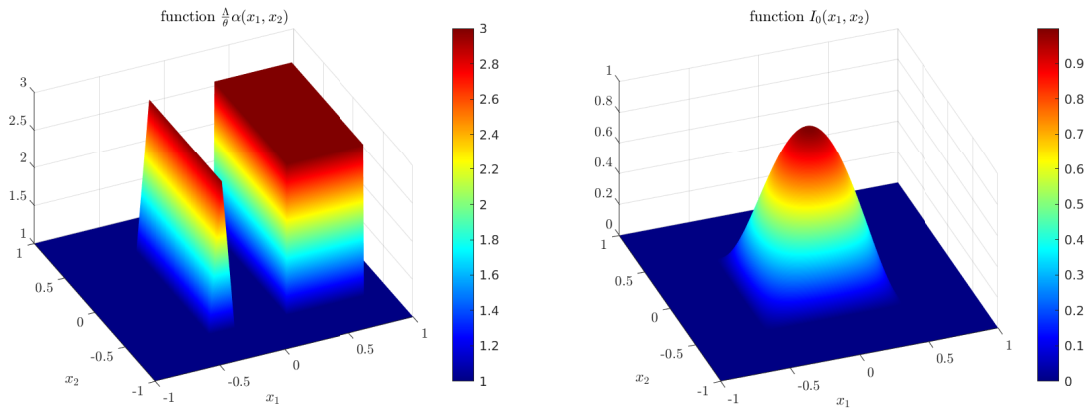
Figure 1: Illustration of Theorem 2.2 in the case i), i.e. , when I_0(\alpha^{-1}(\alpha^*)) > 0 . Parameters of this simulation are: \Lambda = 2 , \theta = 1 , \alpha(x) = 0.5 + (\mathbb{T}_{[-0.4, -0.2]}(x_1) + \mathbb{1}_{[0.2, 0.8]}(x_1)) \mathbb{1}_{[-0.6, 0.6]}(x_2) where x = (x_1, x_2) \in \mathbb{R}^2 and \mathbb{T}_{[-0.4, -0.2]} is the triangular function of height one and support [-0.4, -0.2] , and \gamma = \frac{1}{2\alpha} . Initial condition is given by I_0(dx) = I_0(x_1, x_2) dx where I_0(x_1, x_2) = \mathbb{1}_{[-0.5, 0.5]}(x_1) \cos(\pi x_1) \mathbb{1}_{[-0.5, 0.5]}(x_2) \cos(\pi x_2) . In particular, we have \alpha^* = 3/2 and \alpha^{-1}(\alpha^*) = (\{-0.3\} \cup [0.2, 0.5]) \times [-0.5, 0.5] .
