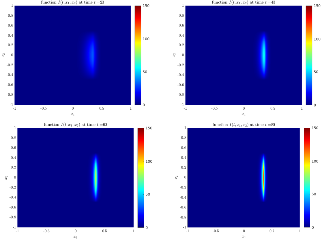
Figure 6: Illustration of Theorem 2.2 in the case ii), i.e. , when I_0(\alpha^{-1}(\alpha^*)) = 0 . Function x \rightarrow I(t, x) at time t = 20, 40, 60 and 80 . The function I asymptotically converges towards a singular measure.
