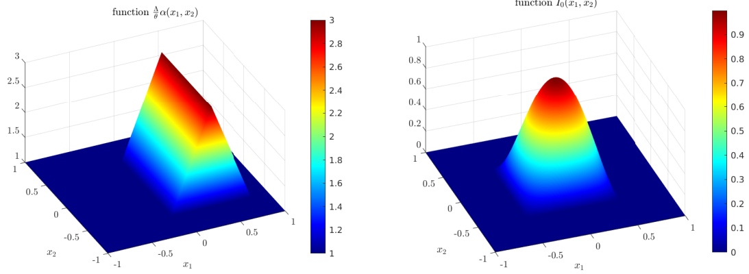
Figure 4: Illustration of Theorem 2.2 in the case ii), i.e. , when I_0(\alpha^{-1}(\alpha^*)) = 0 . Parameters of this simulation are: \Lambda = 2 , \theta = 1 , \alpha(x) = 0.5 + \mathbb{T}_{[-0.1, 0.8]}(x_1) \mathbb{1}_{[-0.5, 0.5]}(x_2) where x = (x_1, x_2) \in \mathbb{R}^2 and \mathbb{T}_{[-0.1, 0.5]} is the triangular function of height one and support [-0.1, 0.5] , \gamma = \frac{1}{2\alpha} . Initial condition is given by I_0(dx) = I_0(x_1, x_2) dx where I_0(x) = \mathbb{1}_{[-0.5, 0.5]}(x_1) \cos(\pi x_1) \mathbb{1}_{[-0.5, 0.5]}(x_2) \cos(\pi x_2) . In particular, \alpha^* = 3/2 and \alpha^{-1}(\alpha^*) = \{0.35\} \times [-0.5, 0.5] .
