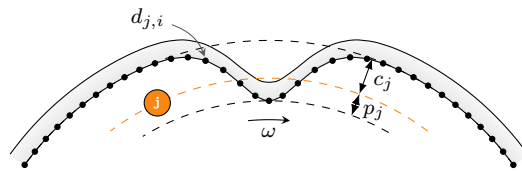
Figure 3 – Casing distortion (□) in front of the j -th boundary node (●).
