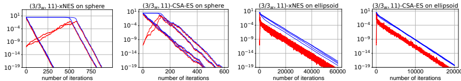
Figure 2: Four independent runs of (\mu/\mu_w, \lambda) -xNES and (\mu/\mu_w, \lambda) -CSA1-ES (without cumulation) as presented in Section 2.1 on the functions x \mapsto \|x\|^2 (first two figures) and x \mapsto \sum_{i=1}^n 10^{3\frac{i-1}{n-1}} x_i^2 (last two figures). Illustration of \|X_k\| in blue and \sigma_k in red where k is the number of iterations, \mu = 3 , \lambda = 11 and w_i = 1/\mu . Initializations: \sigma_0 equals to 10^{-11} in two runs and 1 in the two other runs, X_0 is the all-ones vector in dimension 10.
