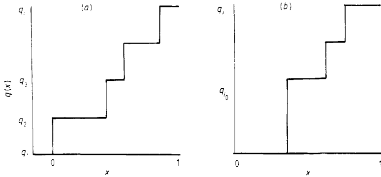
Figure 1. (a) Shape of q(x) when the a_i and \log \alpha_i satisfy condition (16) for T_{i-1} < T < T_i . (b) Shape of q(x) when the sequence a_i/\log \alpha_i has a maximum for T_{i-1} < T < T_i , with i > i_0 . The value of i_0 is given by formula (20).
