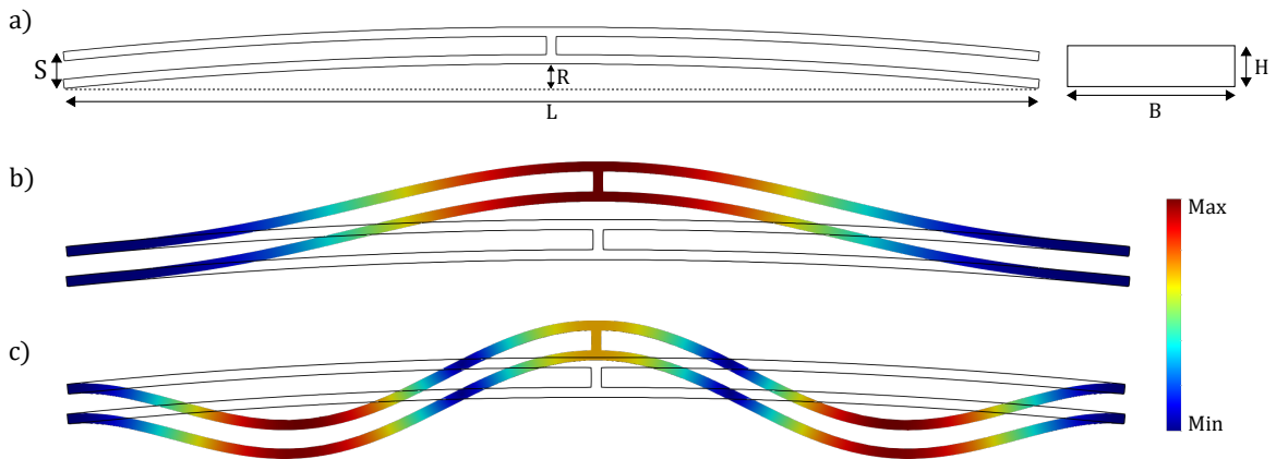
Fig. 8 Arch view along the \mathbf{e}_1 - \mathbf{e}_2 plane on the left and arch beam section geometry on the right (a). The geometrical dimensions of the arch are B = 20 \mu\text{m} , H = 5 \mu\text{m} , L = 530 \mu\text{m} , R = 13.4 \mu\text{m} , and S = 20 \mu\text{m} . S size includes the beams thickness. Modes that satisfy the 1:2 internal resonance condition are mode 1 (b) and mode 6 (c). The colormap reports the magnitude of the displacement field. The deformation of the structure is amplified to improve the visualisation of the field.
