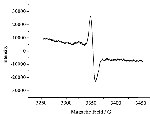
Figure 1. ESR signal of a cross-linked P4VP sample for a 148 kGy integrated dose with a VARIAN E Line spectrometer at a modulation frequency of 100 kHz, microwave frequency 9.3 GHz, mass of polymer = 30 mg.
