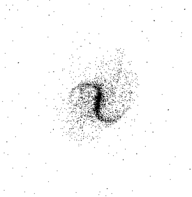
FIG. 12. Barred spiral from numerical simulation (1992: 2 \times 10,000 points).
