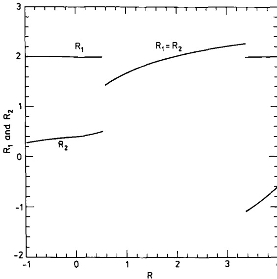
Fig. 4. The solutions R_1(R) and R_2(R) of the saddle point equation (55) for K=2 and E=3 as a function of R . Near the stable fixed point A , the saddle point is symmetric: R_1(R) = R_2(R) , while for larger and smaller values of R the symmetry is broken, R_1(R) \neq R_2(R) .
