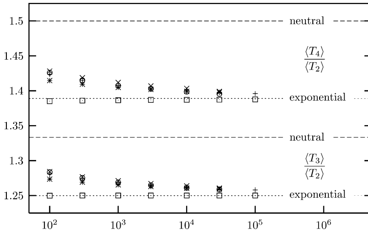
Fig. 2 – Ratios \langle T_3 \rangle / \langle T_2 \rangle and \langle T_4 \rangle / \langle T_2 \rangle vs. N , for the same models (same symbols) as in fig. 1. The dashed lines represent the neutral case eq. (1), and the dotted lines correspond to eq. (3), i.e. Model B with \psi(\epsilon) = e^{-\epsilon} .
